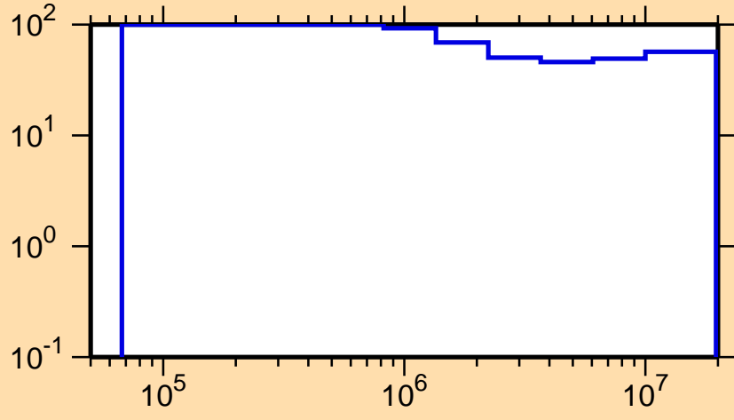
\Delta\sigma/\sigma vs. E for ^{245}\text{Es}(n,\text{inel.})
