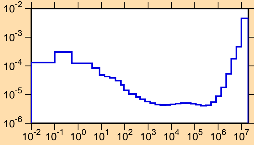
\sigma vs. E for ^{245}\text{Es}(n,\alpha)
