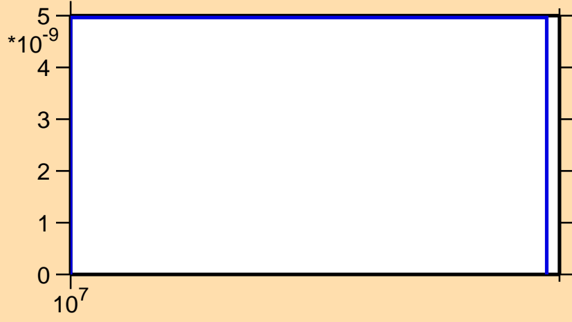
\sigma vs. E for ^{245}\text{Es} (mt 45)
