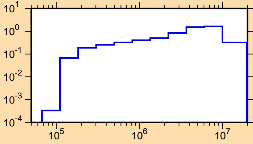
\sigma vs. E for ^{245}\text{Es}(n,\text{inel.})
