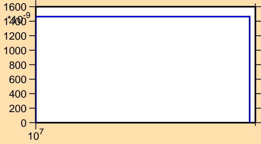
\sigma vs. E for ^{245}\text{Es}(n,2np)
