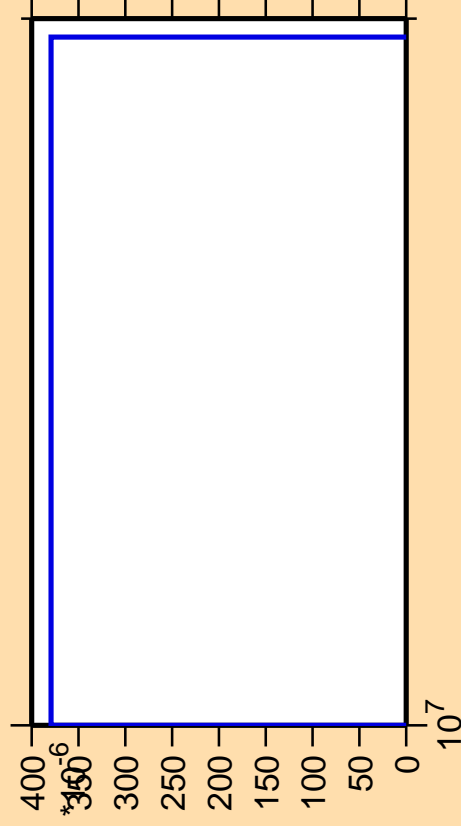
\Delta\sigma/\sigma vs. E for ^{245}\text{Es}(n,3n\alpha)
