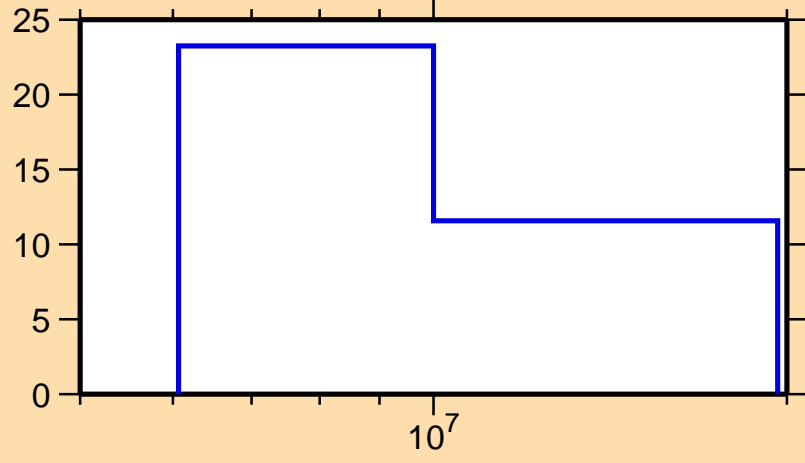
\Delta\sigma/\sigma vs. E for ^{245}\text{Es}(n,\text{el.})
