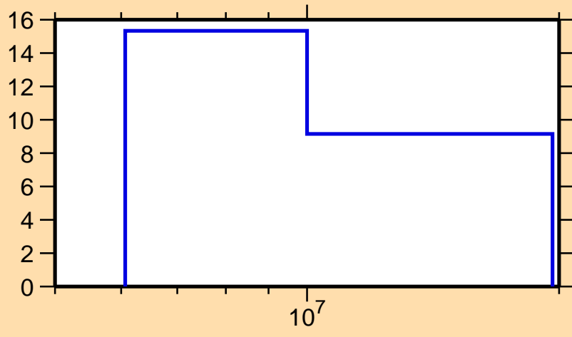
\Delta\sigma/\sigma vs. E for ^{245}\text{Es}(n,\text{tot.})
