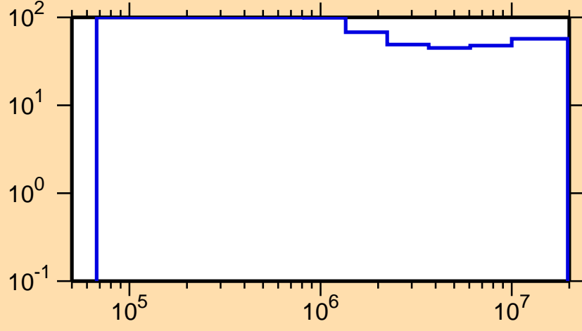
\Delta\sigma/\sigma vs. E for ^{245}\text{Es}(n,n\text{cont.})
