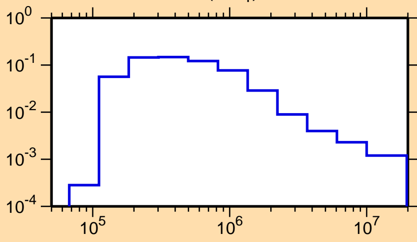
\sigma vs. E for ^{245}\text{Es}(n,n_1)
