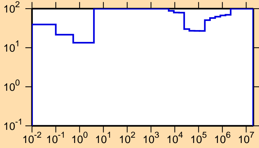
\Delta\sigma/\sigma vs. E for ^{245}\text{Es}(n,\gamma)
