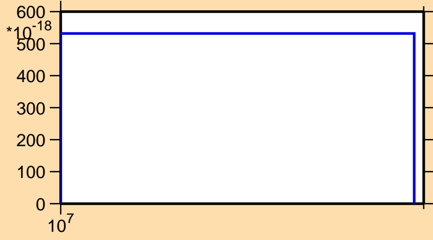
\sigma vs. E for ^{245}\text{Es}(n,3n\alpha)
