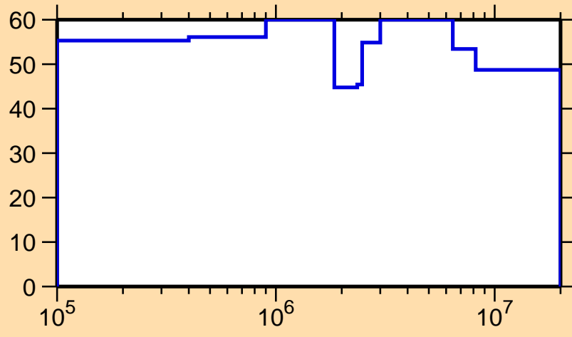
\Delta\sigma/\sigma vs. E for ^{245}\text{Es}(n,n_1)
