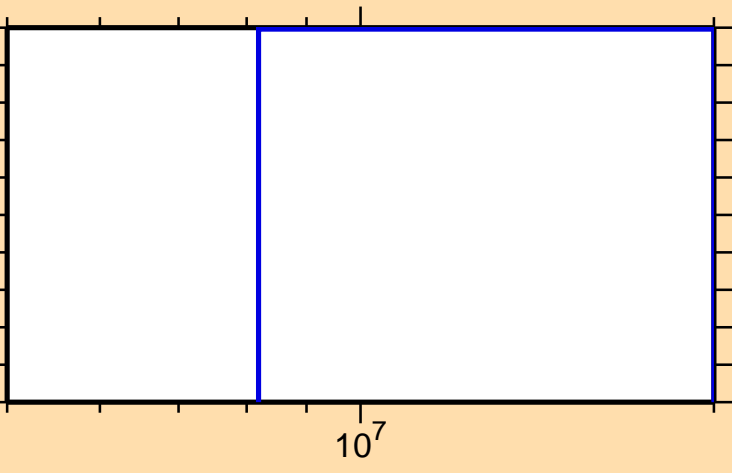
\sigma vs. E for ^{245}\text{Es}(n,\text{He3})
