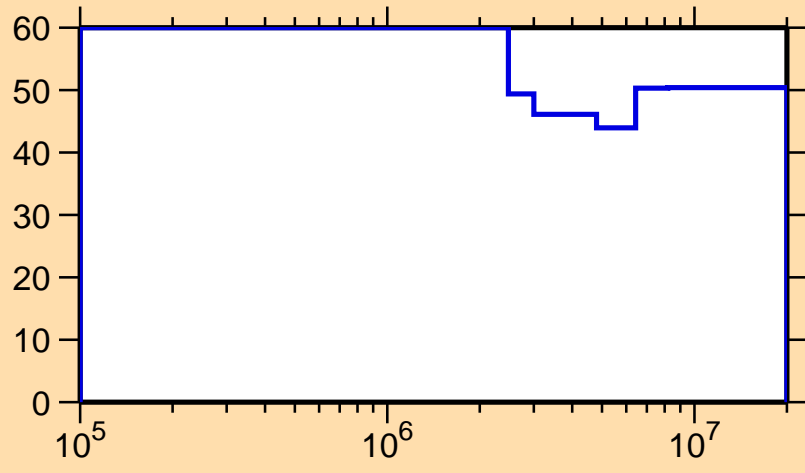
\Delta\sigma/\sigma vs. E for ^{245}\text{Es}(n,n\text{cont.})
