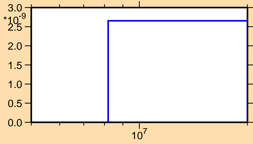
\sigma vs. E for ^{245}\text{Es}(n,p\alpha)
