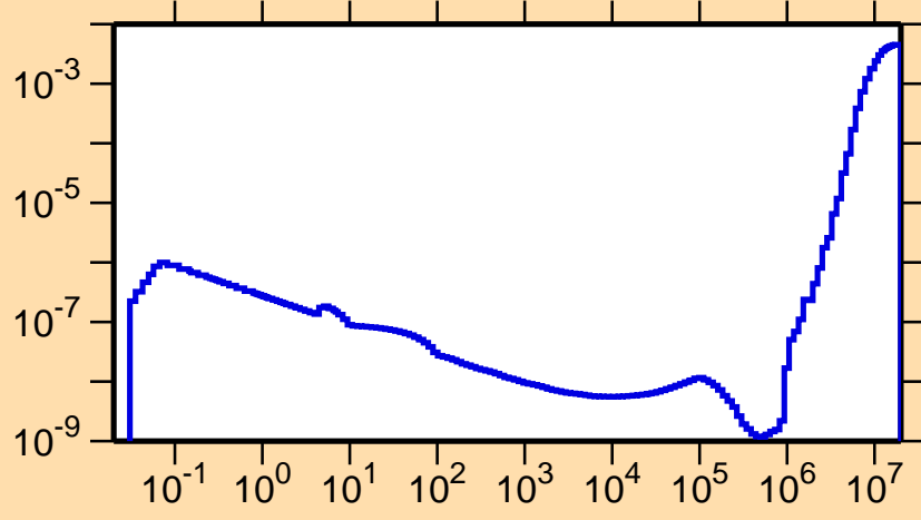
\sigma vs. E for ^{246}\text{Es}(n,p)
