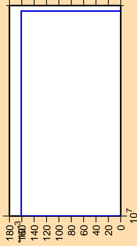
\Delta\sigma/\sigma vs. E for ^{246}\text{Es} (mt 45)
