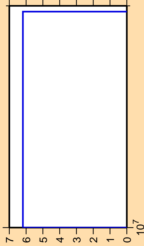
\Delta\sigma/\sigma vs. E for ^{246}\text{Es}(\text{mt117})
