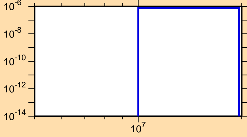
\sigma vs. E for ^{246}\text{Es}(n,nd)
