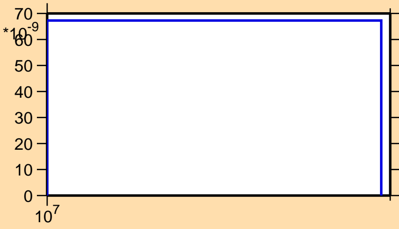
\sigma vs. E for ^{246}\text{Es}(n,2np)
