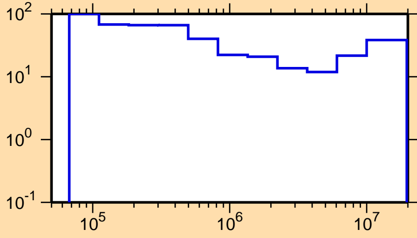
\Delta\sigma/\sigma vs. E for ^{246}\text{Es}(n,n\text{cont.})
