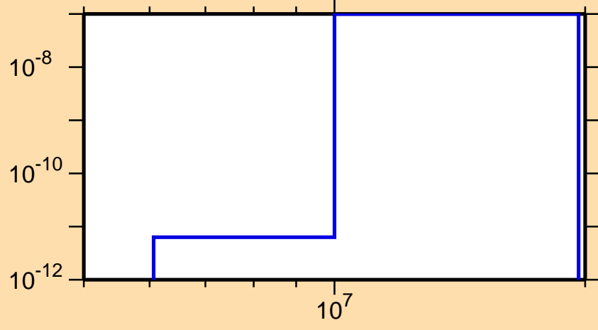
\sigma vs. E for ^{246}\text{Es}(n,2n\alpha)
