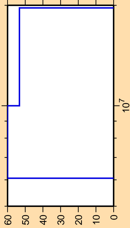
\Delta\sigma/\sigma vs. E for ^{246}\text{Es}(n,n_1)
