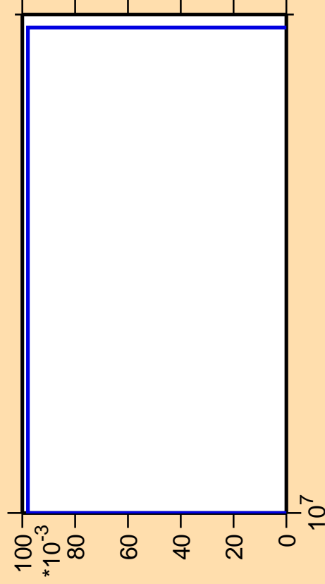
\Delta\sigma/\sigma vs. E for ^{246}\text{Es}(n,3n\alpha)
