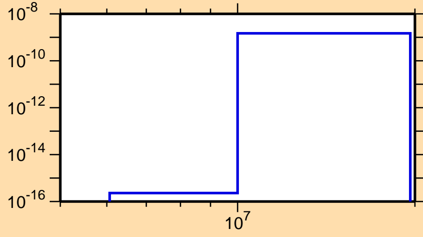
\sigma vs. E for ^{246}\text{Es}(n,\text{He3})
