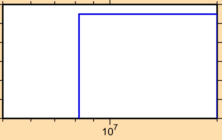
\sigma vs. E for ^{246}\text{Es}(n,2np)
