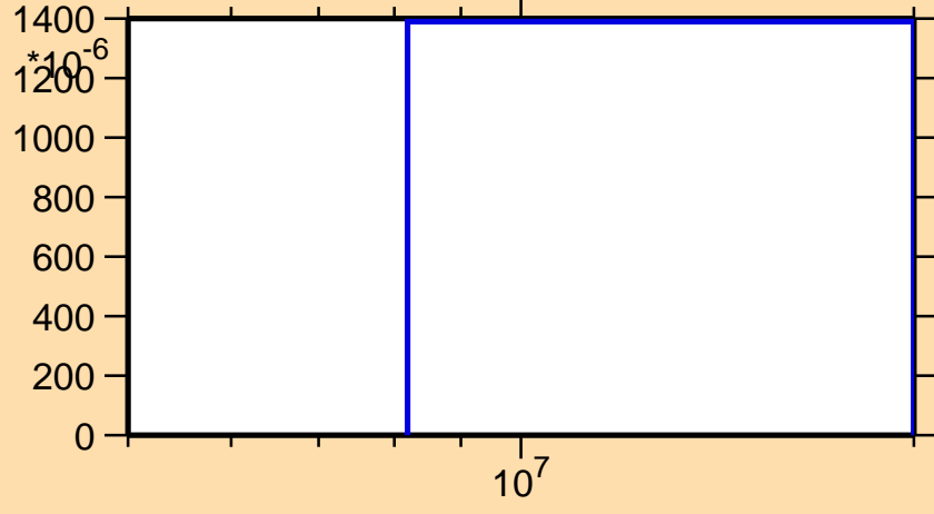
\sigma vs. E for ^{246}\text{Es}(n,3n)
