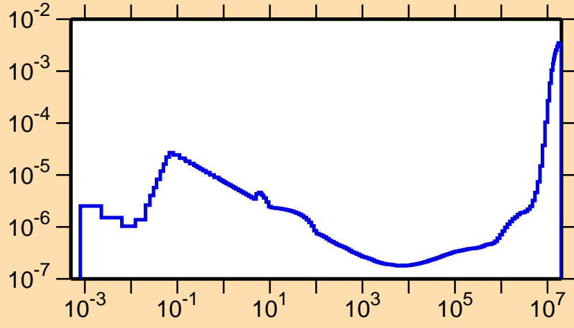
\sigma vs. E for ^{247}\text{Es}(n,\alpha)
