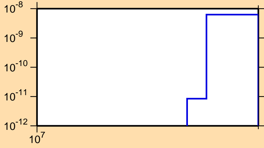
\sigma vs. E for ^{247}\text{Es}(n,3n\alpha)
