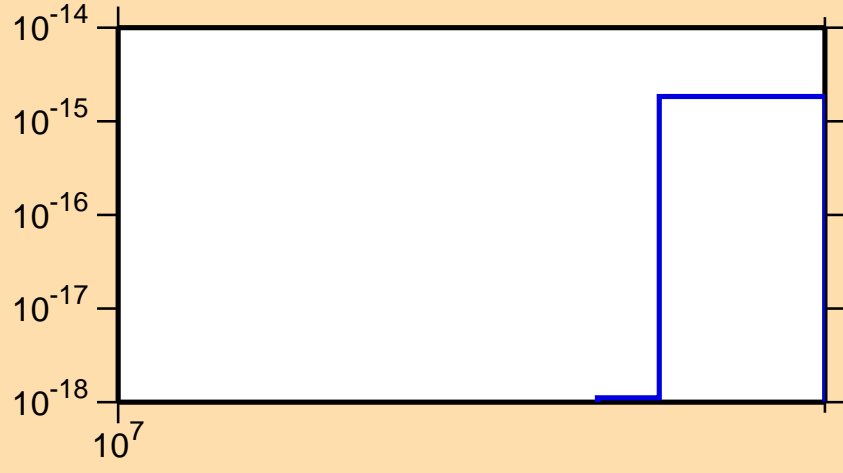
\sigma vs. E for ^{247}\text{Es} (mt 11)
