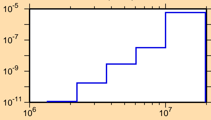
\sigma vs. E for ^{247}\text{Es}(n,n\alpha)
