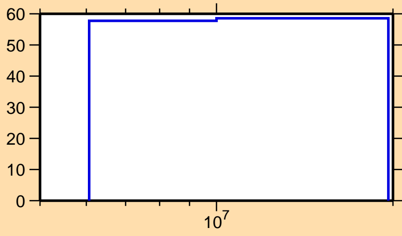
\Delta\sigma/\sigma vs. E for ^{247}\text{Es}(n,2n)
