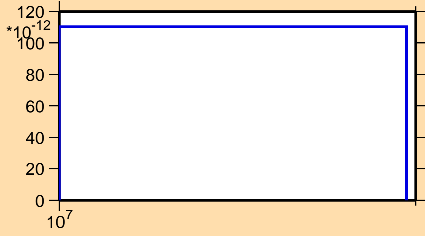
\sigma vs. E for ^{247}\text{Es}(n,\text{He3})
