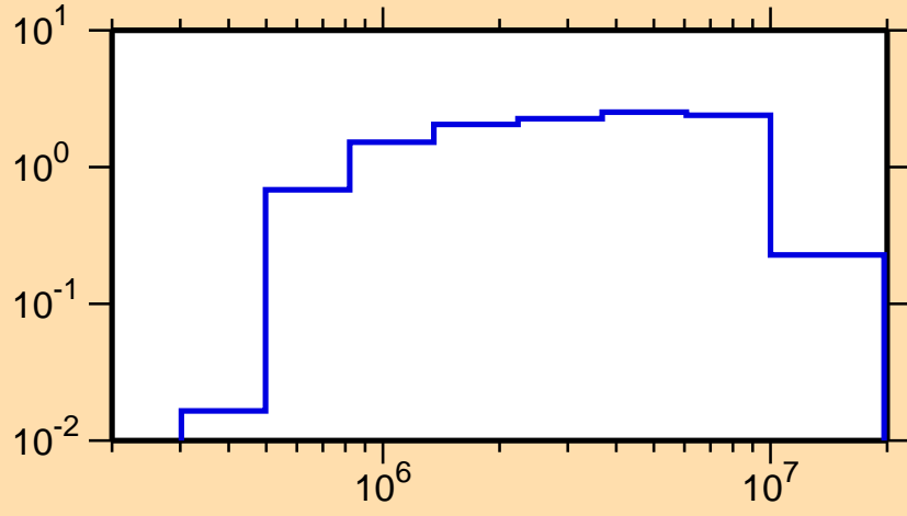
\sigma vs. E for ^{247}\text{Es}(n,\text{inel.})
