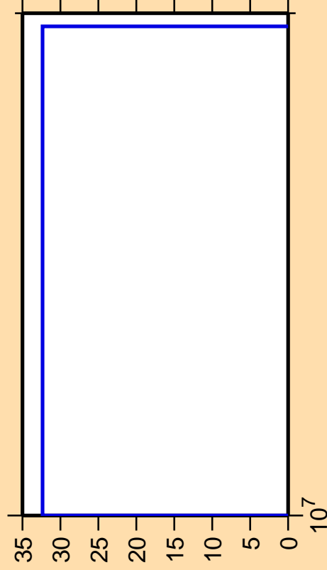
\Delta\sigma/\sigma vs. E for ^{247}\text{Es}(n,3n\alpha)
