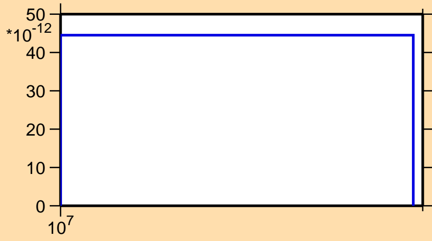
\sigma vs. E for ^{247}\text{Es}(n,3n\alpha)
