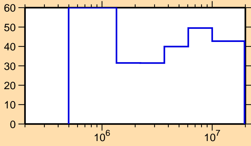
\Delta\sigma/\sigma vs. E for ^{247}\text{Es}(n,n\text{cont.})
