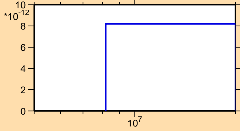
\sigma vs. E for ^{247}\text{Es}(n,nd)
