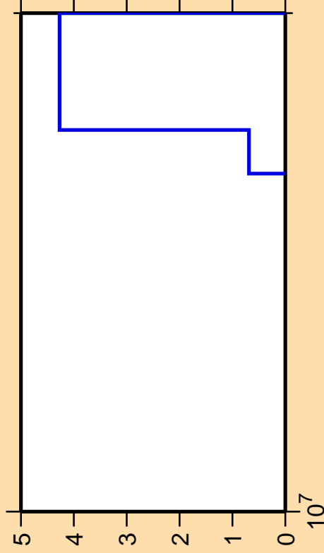
\Delta\sigma/\sigma vs. E for ^{248}\text{Es} (mt 45)
