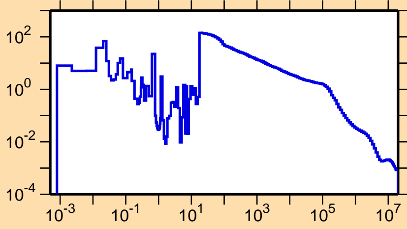
\sigma vs. E for ^{248}\text{Es}(n,\gamma)
