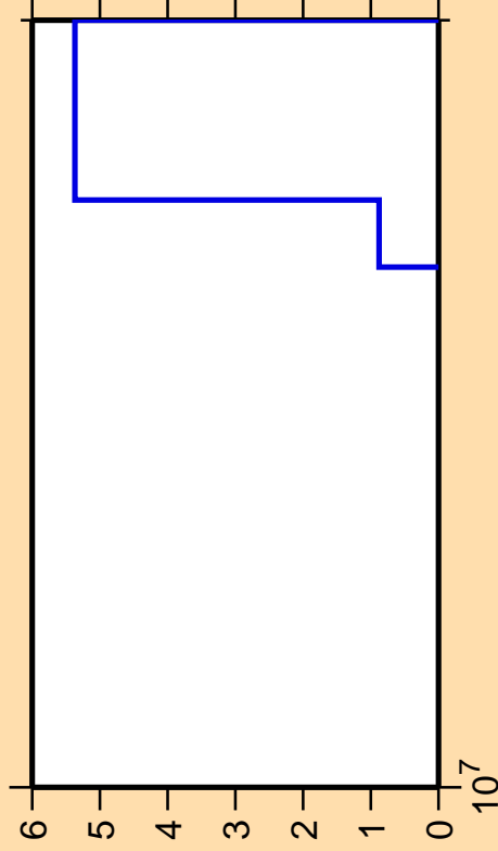
\Delta\sigma/\sigma vs. E for ^{248}\text{Es}(\text{mt117})
