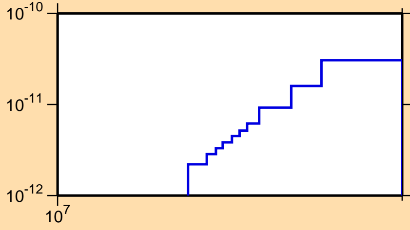
\sigma vs. E for ^{248}\text{Es}(n,p\alpha)
