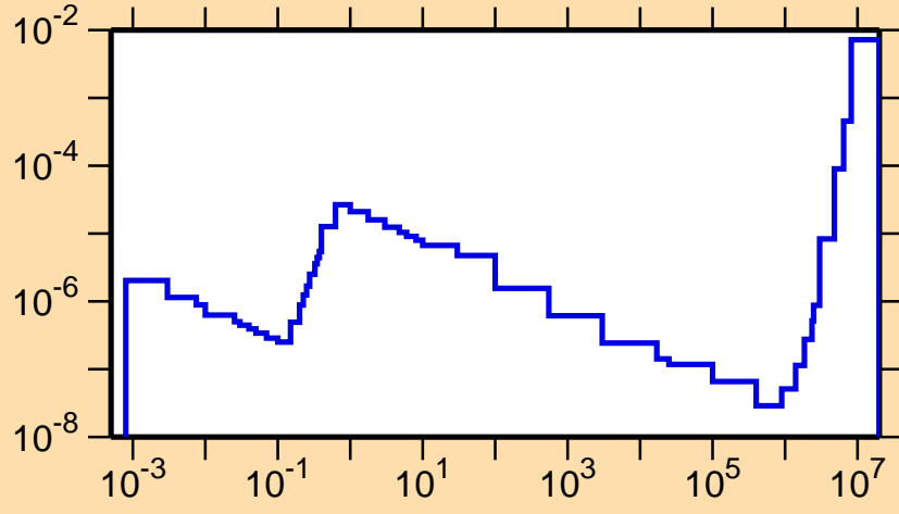
\sigma vs. E for ^{248}\text{Es}(n,p)
