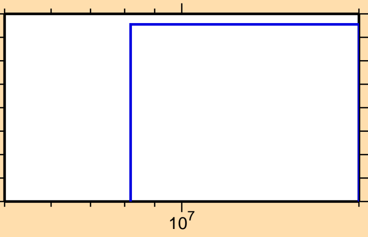
\sigma vs. E for ^{248}\text{Es} (mt 11)
