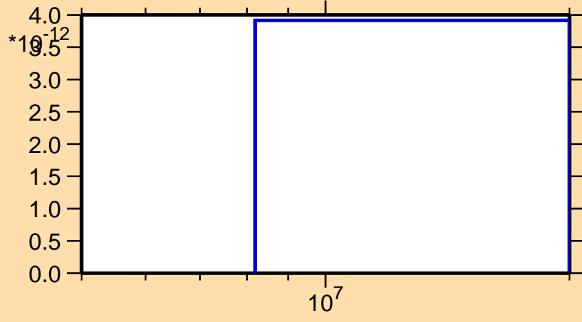
\sigma vs. E for ^{248}\text{Es}(n,p\alpha)
