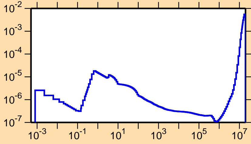
\sigma vs. E for ^{249}\text{Es}(n,\alpha)
