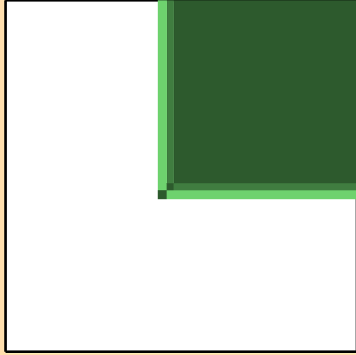
\sigma vs. E for ^{249}\text{Es}(n,3n)
