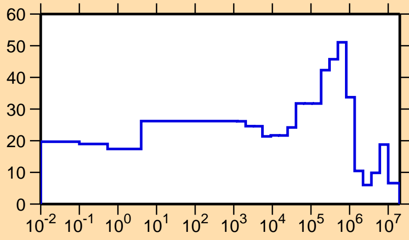
\Delta\sigma/\sigma vs. E for ^{249}\text{Es}(n,el.)
