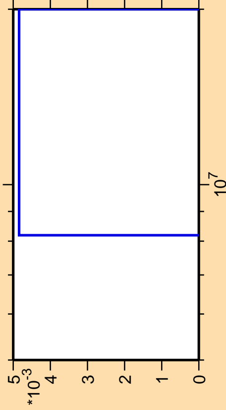
\Delta\sigma/\sigma vs. E for ^{249}\text{Es}(\text{mt } 11)
