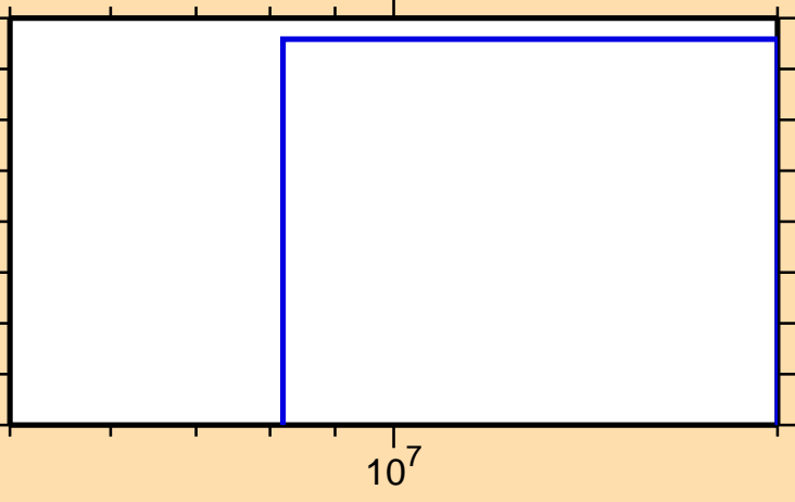
\sigma vs. E for ^{249}\text{Es}(n,\text{He3})
