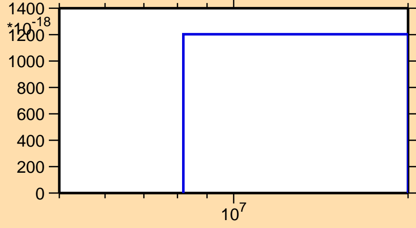
\sigma vs. E for ^{249}\text{Es}(\text{mt } 11)
