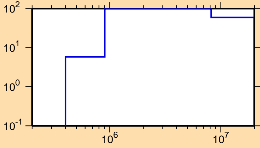
\Delta\sigma/\sigma vs. E for ^{249}\text{Es}(n,p)
