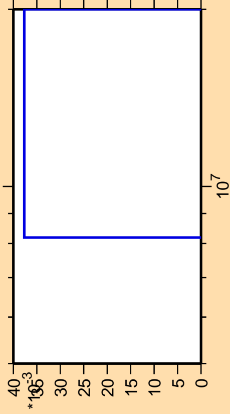
\Delta\sigma/\sigma vs. E for ^{249}\text{Es} (mt 34)
