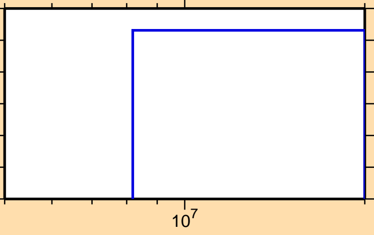
\sigma vs. E for ^{249}\text{Es}(n,nt)
