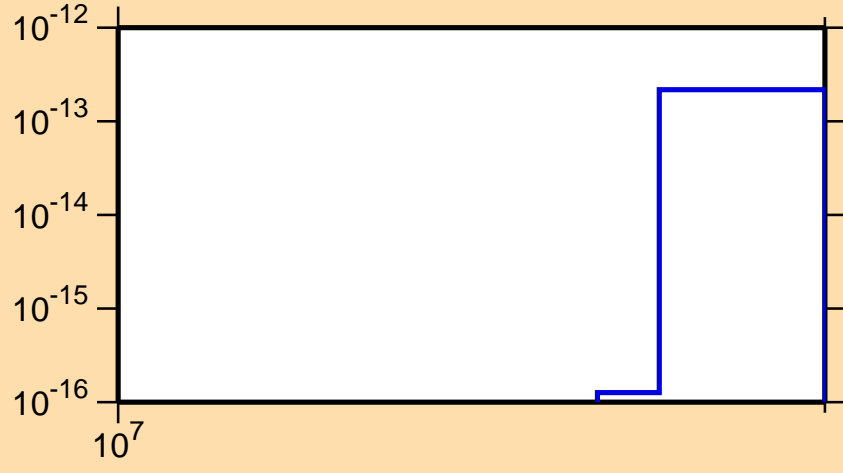
\sigma vs. E for ^{250}\text{Es} (mt 11)
