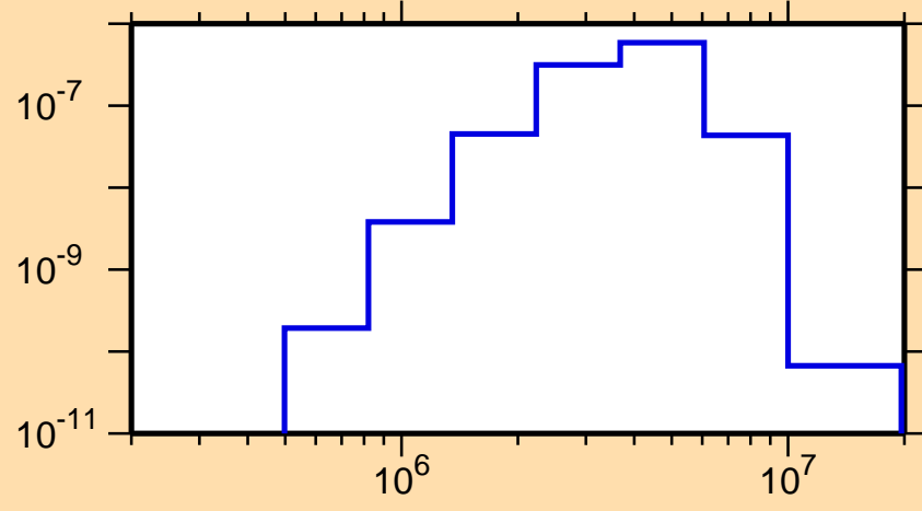
\sigma vs. E for ^{250}\text{Es}(n,n_3)
