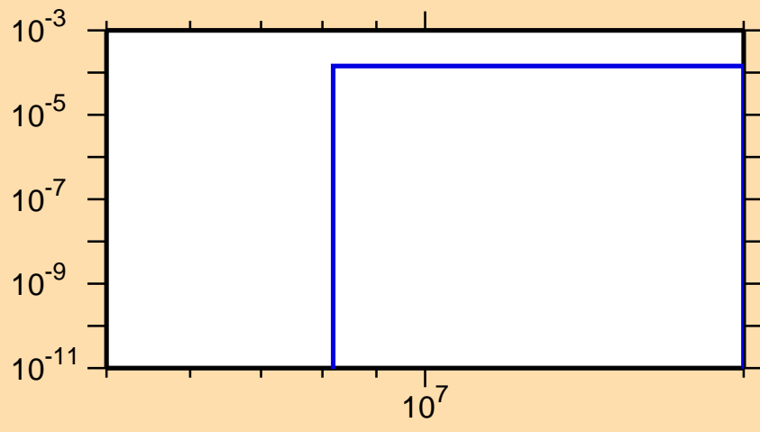
\sigma vs. E for ^{250}\text{Es}(n,t)
