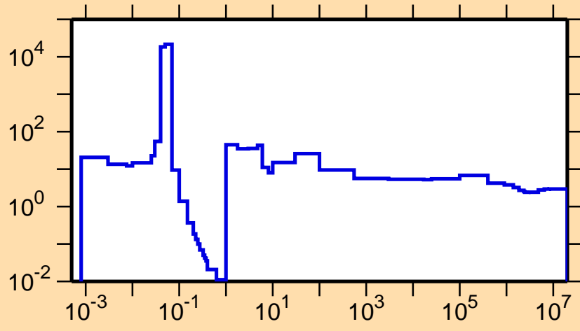
\sigma vs. E for ^{250}\text{Es}(n,\text{nonel.})
