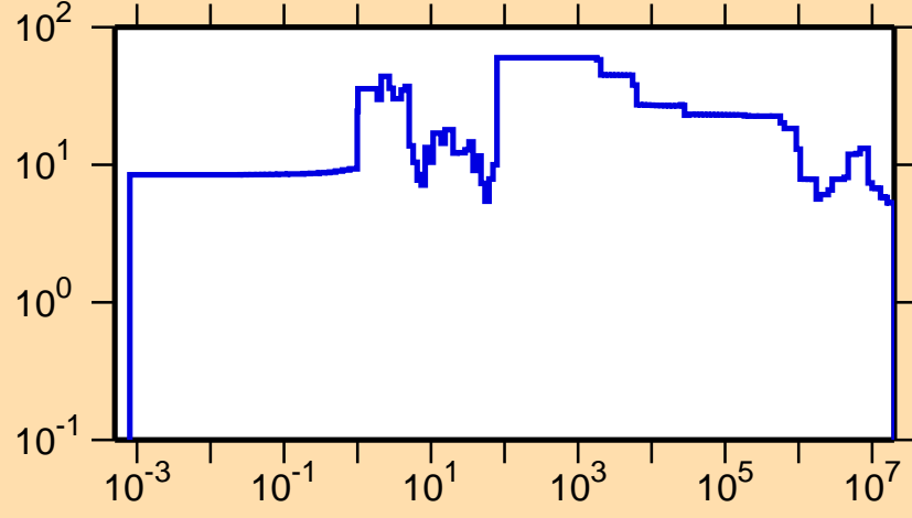
\Delta\sigma/\sigma vs. E for ^{251}\text{Es}(n,el.)
