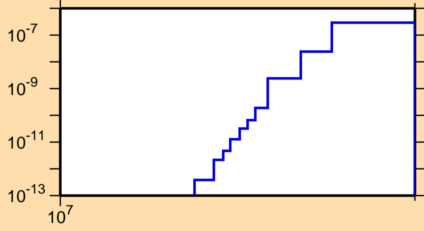
\sigma vs. E for ^{251}\text{Es}(n,nd)
