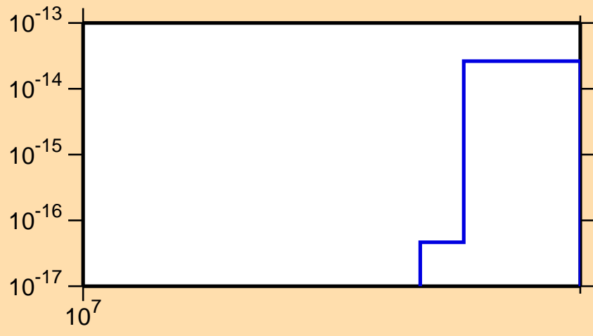
\sigma vs. E for ^{251}\text{Es} (mt 11)
