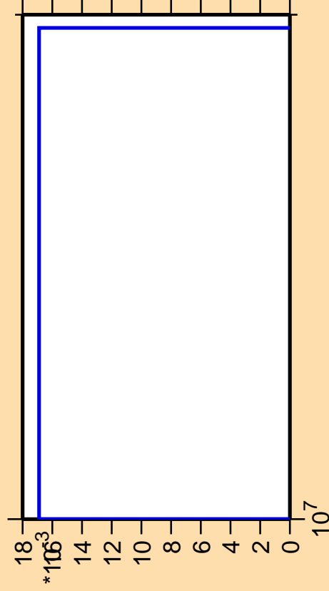
\Delta\sigma/\sigma vs. E for ^{251}\text{Es}(n,3n\alpha)
