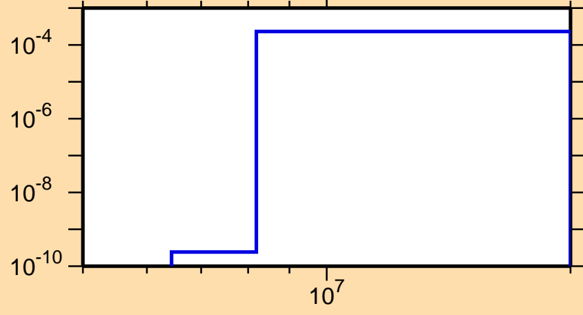
\sigma vs. E for ^{251}\text{Es}(n,np)
