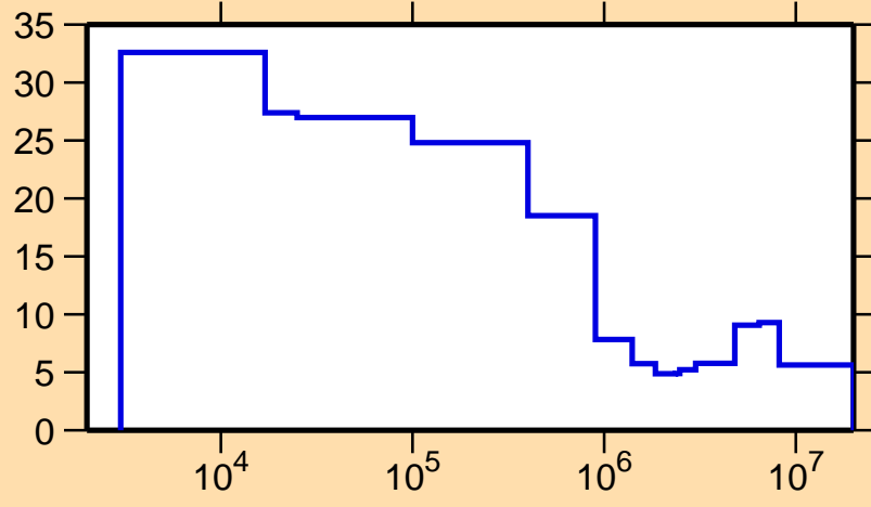
\Delta\sigma/\sigma vs. E for ^{251}\text{Es}(n,\text{tot.})
