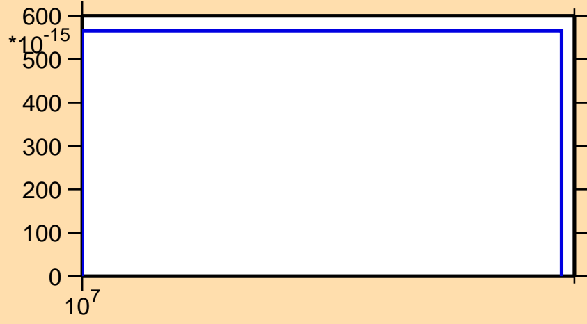
\sigma vs. E for ^{252}\text{Es}(n,3n\alpha)
