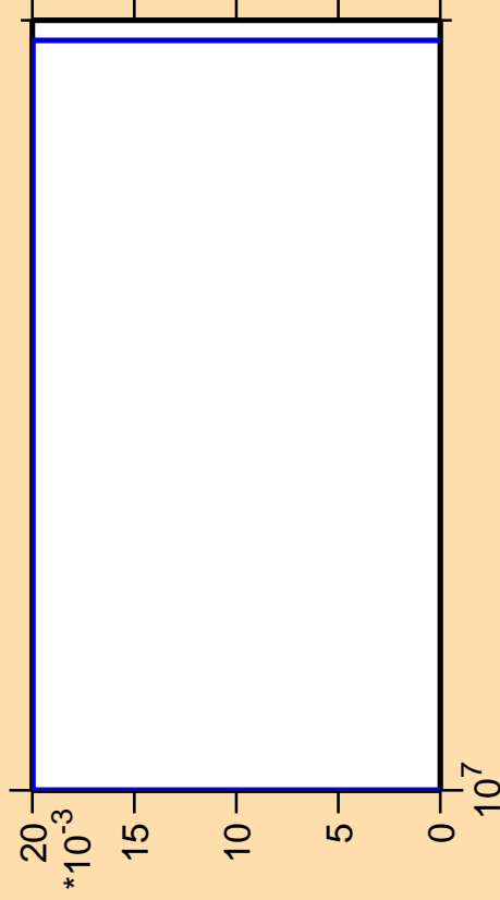
\Delta\sigma/\sigma vs. E for ^{252}\text{Es} (mt 11)
