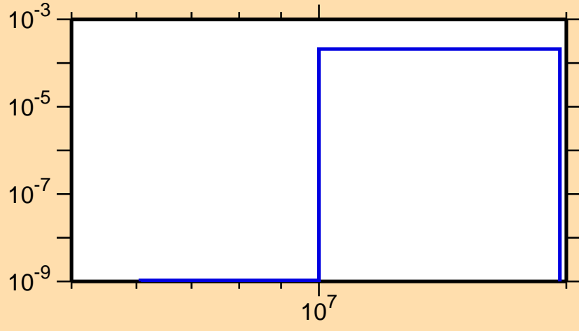
\sigma vs. E for ^{252}\text{Es}(n,np)
