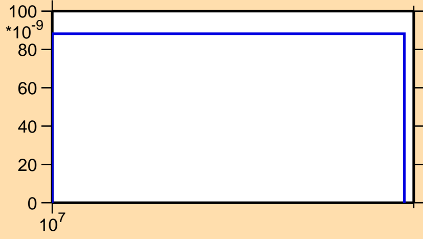
\sigma vs. E for ^{252}\text{Es}(n,2np)
