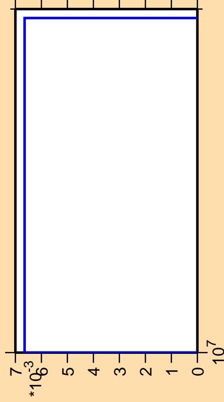
\Delta\sigma/\sigma vs. E for ^{252}\text{Es} (mt 34)
