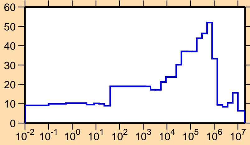
\Delta\sigma/\sigma vs. E for ^{252}\text{Es}(n,el.)
