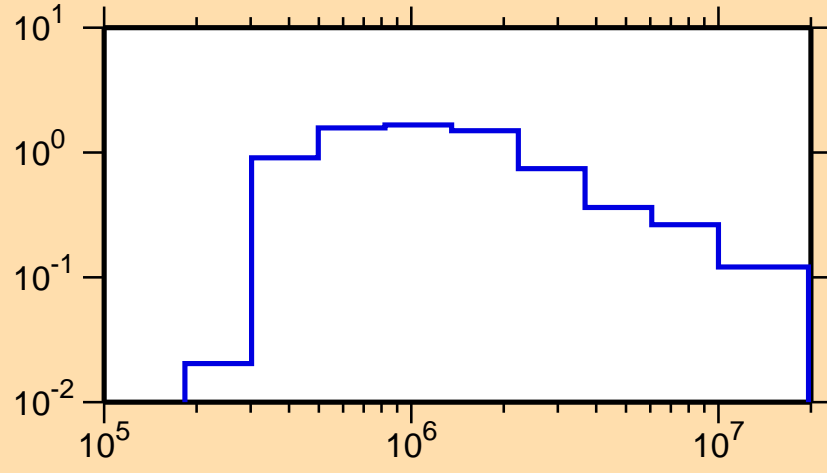
\sigma vs. E for ^{252}\text{Es}(n,n_3)
