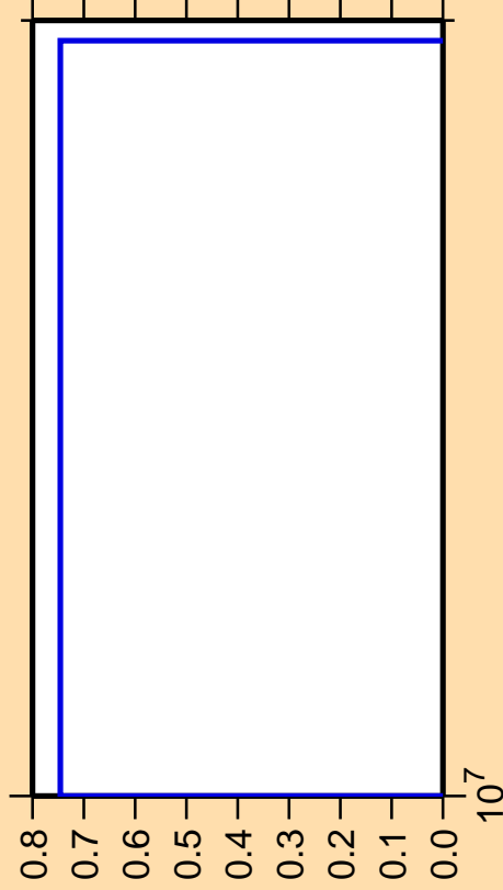
\Delta\sigma/\sigma vs. E for ^{252}\text{Es}(n,3n\alpha)
