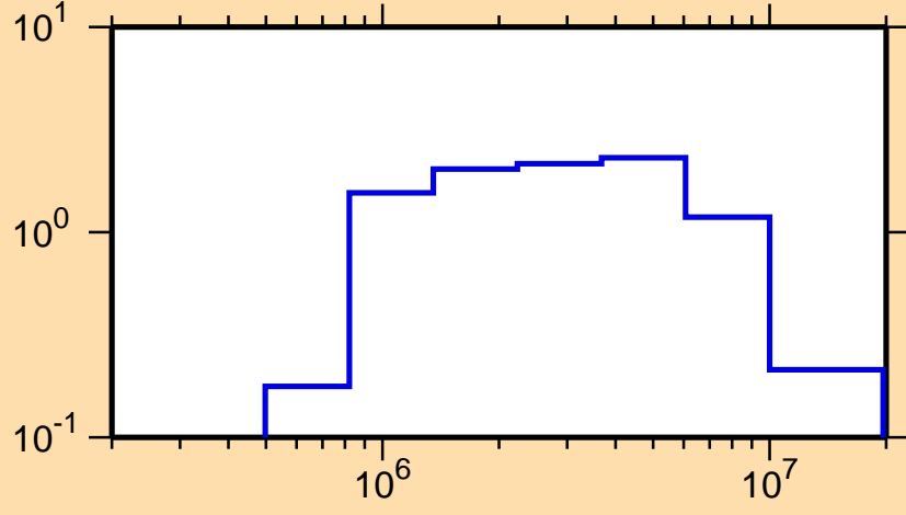
\sigma vs. E for ^{252}\text{Es}(n,n\text{cont.})
