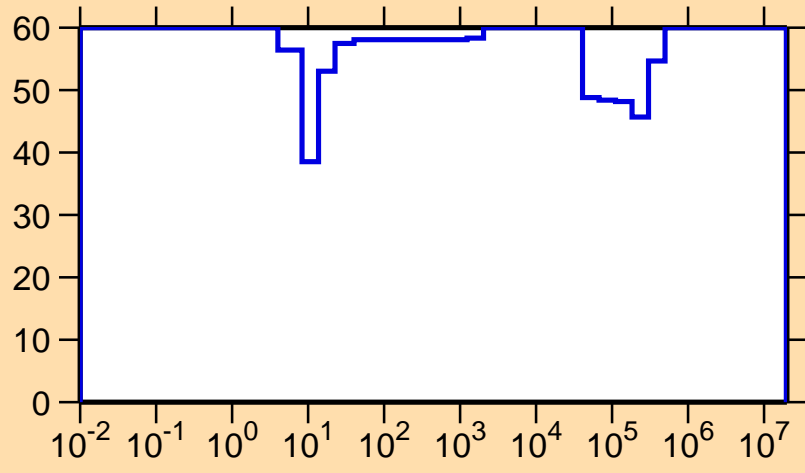
\Delta\sigma/\sigma vs. E for ^{252}\text{Es}(n,\gamma)
