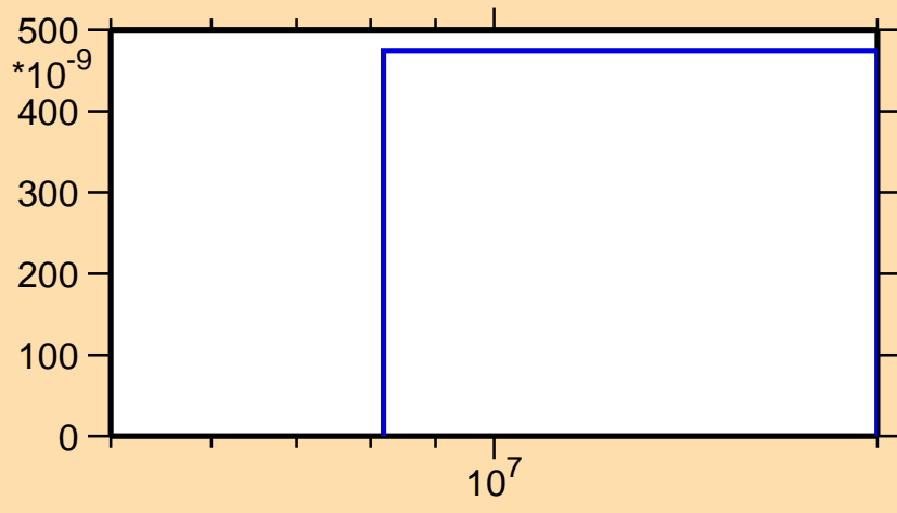
\sigma vs. E for ^{252}\text{Es}(n,nd)
