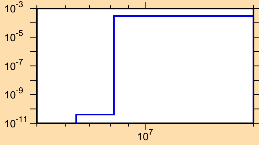
\sigma vs. E for ^{252}\text{Es}(n,d)
