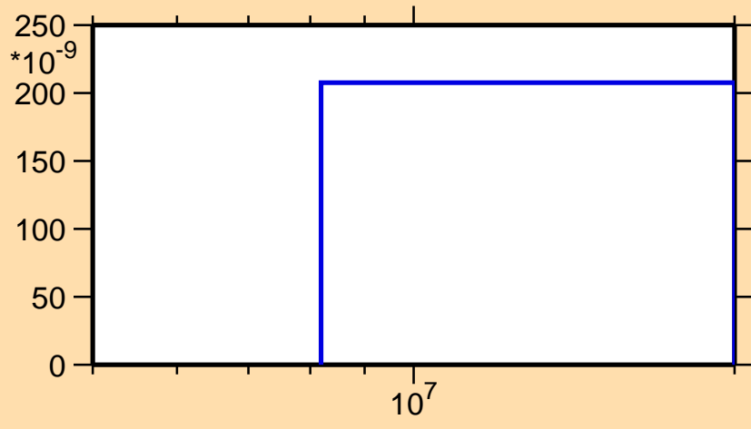
\sigma vs. E for ^{252}\text{Es}(n,nt)
