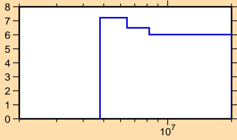
\Delta\sigma/\sigma vs. E for ^{252}\text{Es}(n,\text{nonel.})
