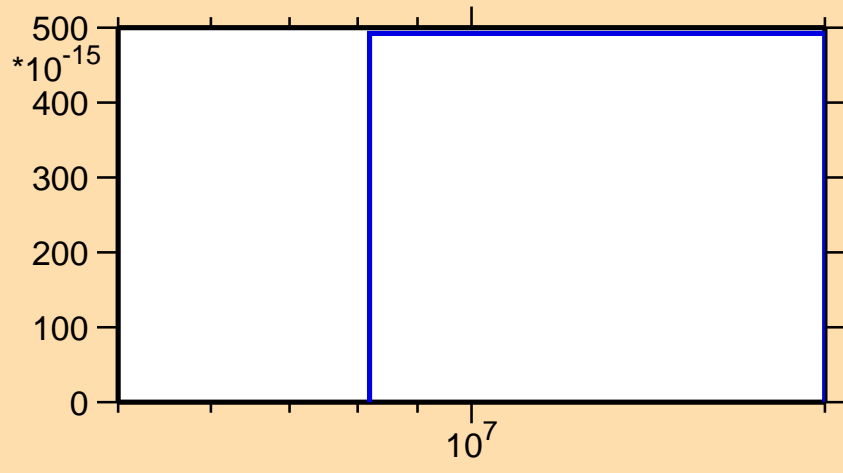
\sigma vs. E for ^{252}\text{Es}(n,3n\alpha)
