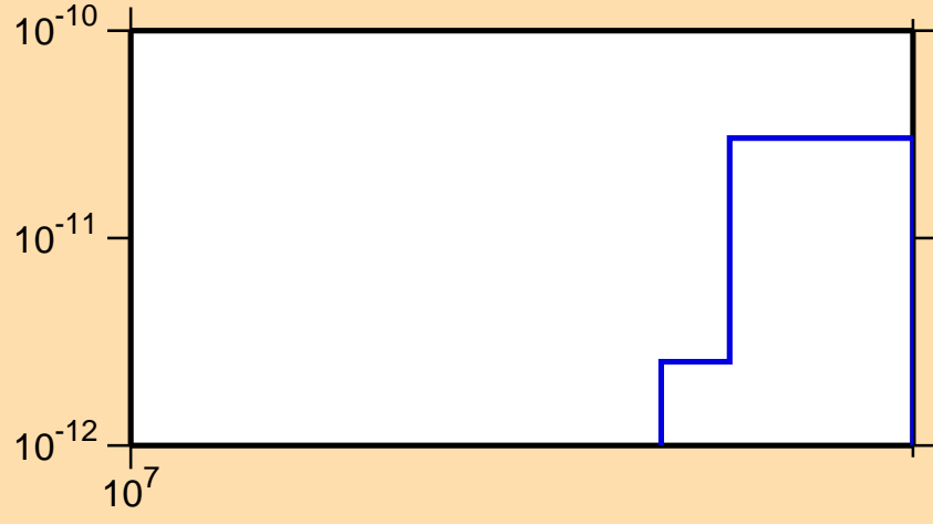
\sigma vs. E for ^{253}\text{Es}(n,3n\alpha)
