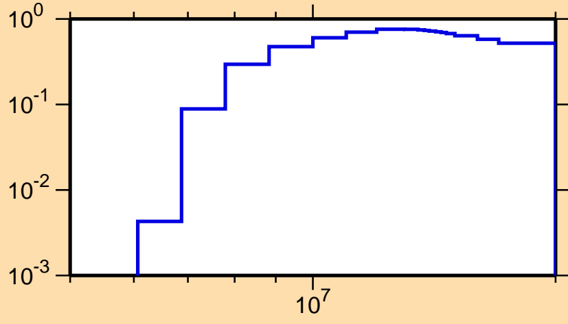
\sigma vs. E for ^{253}\text{Es}(n,2n)
