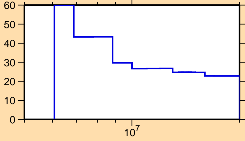
\Delta\sigma/\sigma vs. E for ^{253}\text{Es}(n,\text{inel.})
