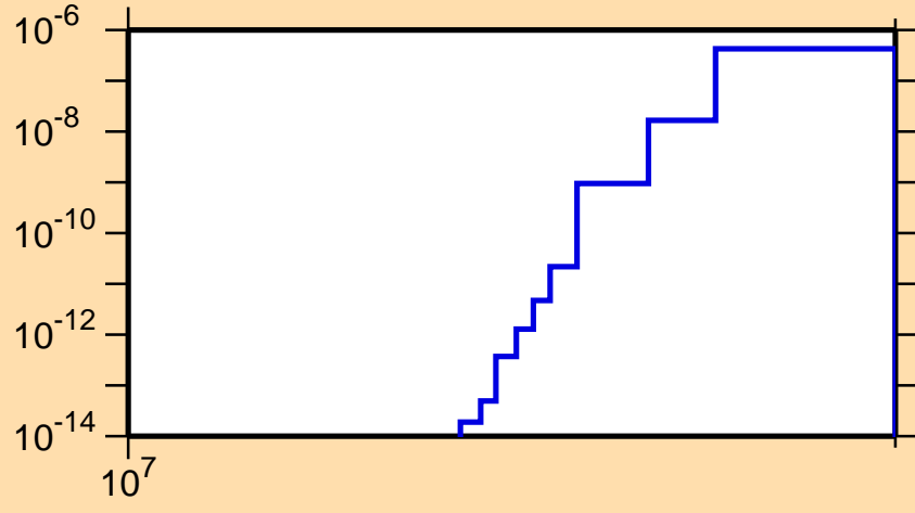
\sigma vs. E for ^{253}\text{Es}(n,2np)
