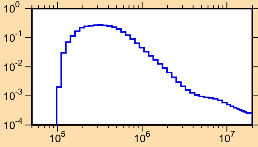
\sigma vs. E for ^{253}\text{Es}(n,n_3)
