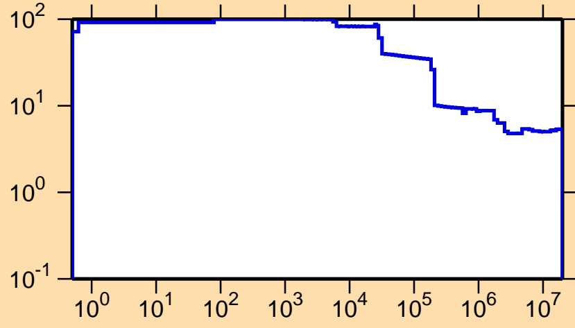
\Delta\sigma/\sigma vs. E for ^{253}\text{Es}(n,\text{nonel.})
