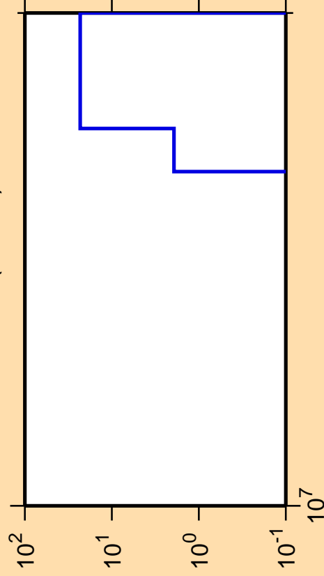
\Delta\sigma/\sigma vs. E for ^{253}\text{Es}(n,3n\alpha)
