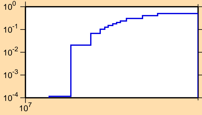
\sigma vs. E for ^{253}\text{Es}(n,3n)
