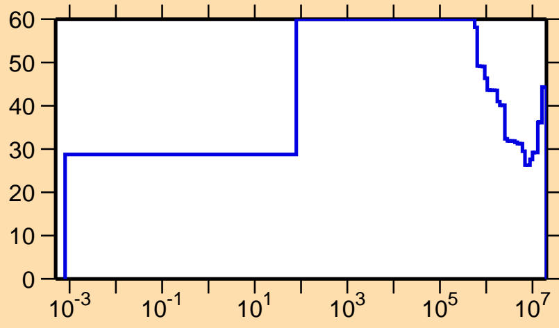
\Delta\sigma/\sigma vs. E for ^{253}\text{Es}(n,f)
