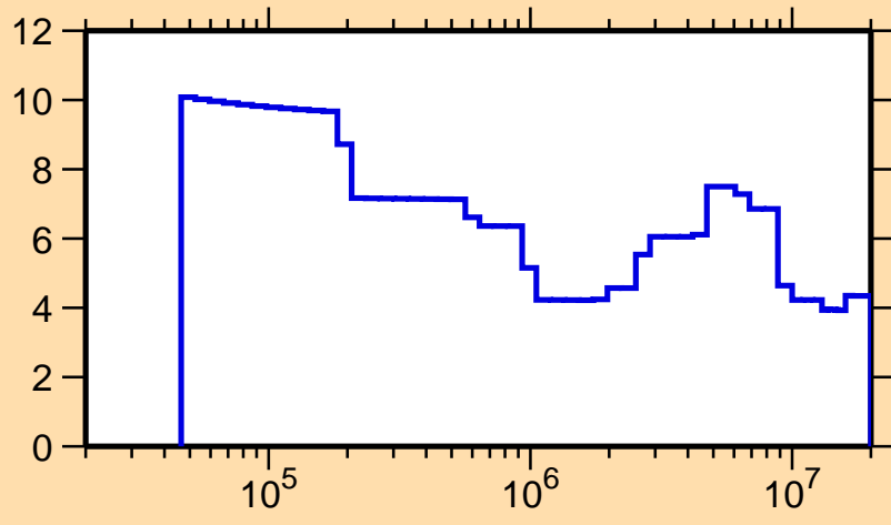
\Delta\sigma/\sigma vs. E for ^{253}\text{Es}(n,\text{tot.})
