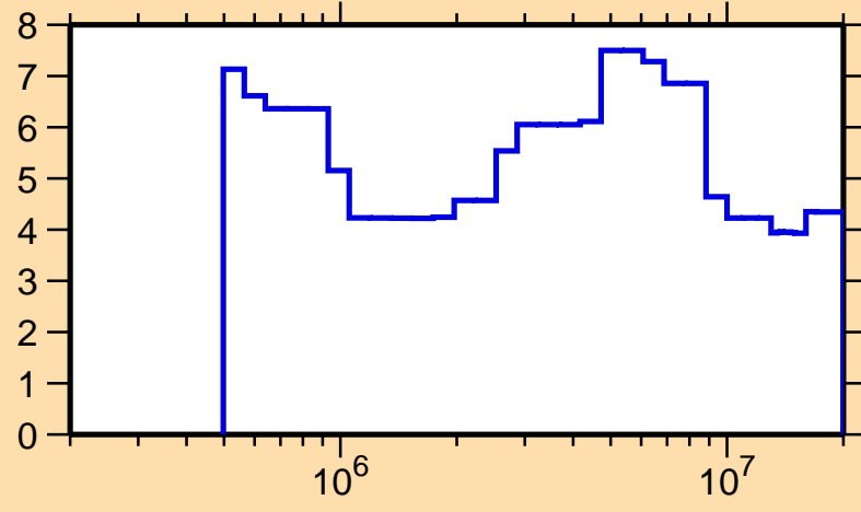
\Delta\sigma/\sigma vs. E for ^{253}\text{Es}(n, \text{tot.})
