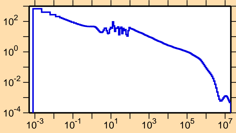
\sigma vs. E for ^{253}\text{Es}(n,\gamma)
