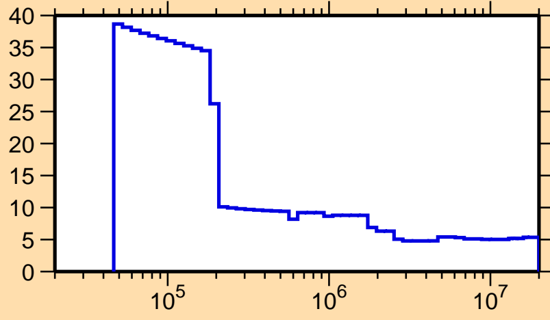
\Delta\sigma/\sigma vs. E for ^{253}\text{Es}(n,\text{nonel.})
