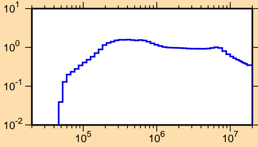
\sigma vs. E for ^{253}\text{Es}(n,\text{inel.})
