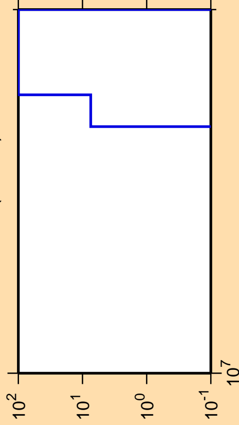
\Delta\sigma/\sigma vs. E for ^{253}\text{Es}(n,\text{He3})
