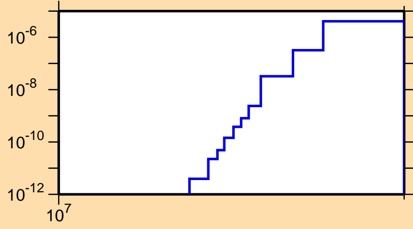
\sigma vs. E for ^{253}\text{Es}(n,nd)
