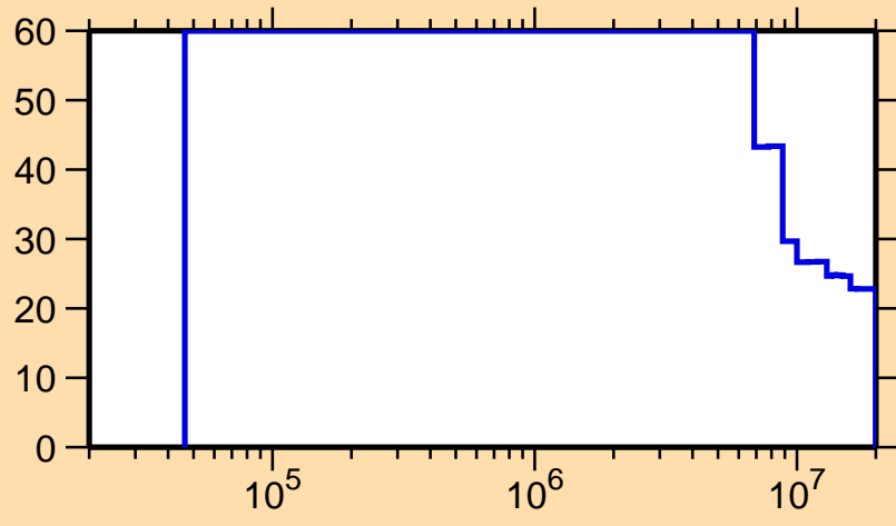
\Delta\sigma/\sigma vs. E for ^{253}\text{Es}(n,\text{inel.})
