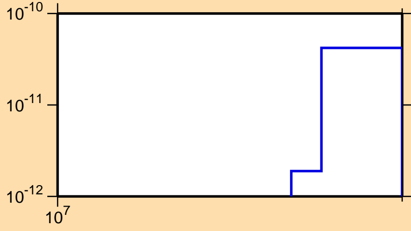
\sigma vs. E for ^{253}\text{Es}(n,\text{He3})
