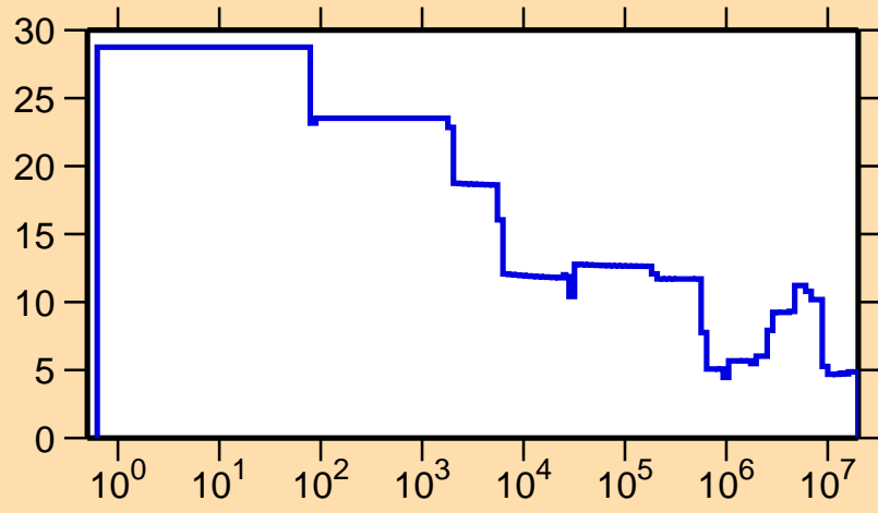
\Delta\sigma/\sigma vs. E for ^{253}\text{Es}(n,\text{el.})
