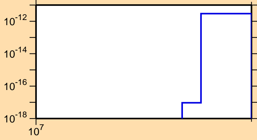
\sigma vs. E for ^{253}\text{Es} (mt 11)
