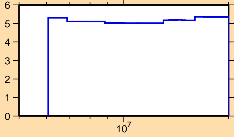
\Delta\sigma/\sigma vs. E for ^{253}\text{Es}(n,\text{nonel.})
