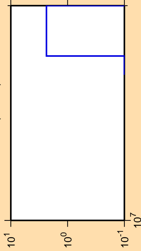
\Delta\sigma/\sigma vs. E for ^{253}\text{Es} (mt 11)
