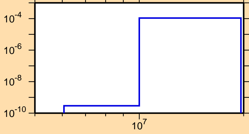
\sigma vs. E for ^{253}\text{Es}(n,np)
