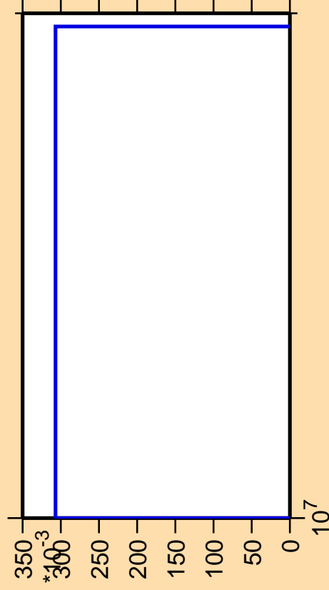
\Delta\sigma/\sigma vs. E for ^{253}\text{Es}(n,3n\alpha)
