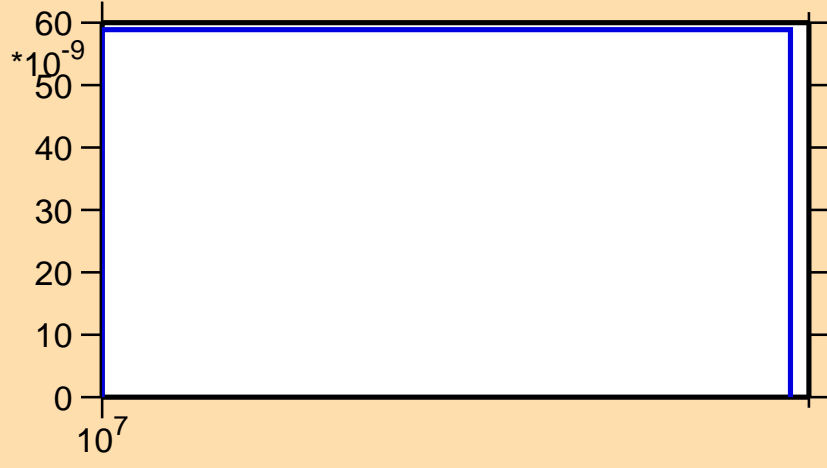
\sigma vs. E for ^{253}\text{Es}(n,nd)
