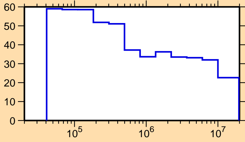
\Delta\sigma/\sigma vs. E for ^{253}\text{Es}(n,n_1)
