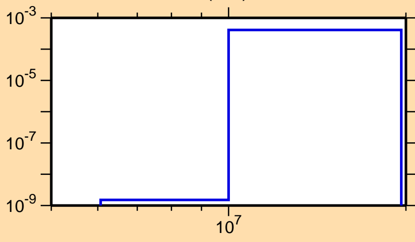
\sigma vs. E for ^{254}\text{Es}(n,d)
