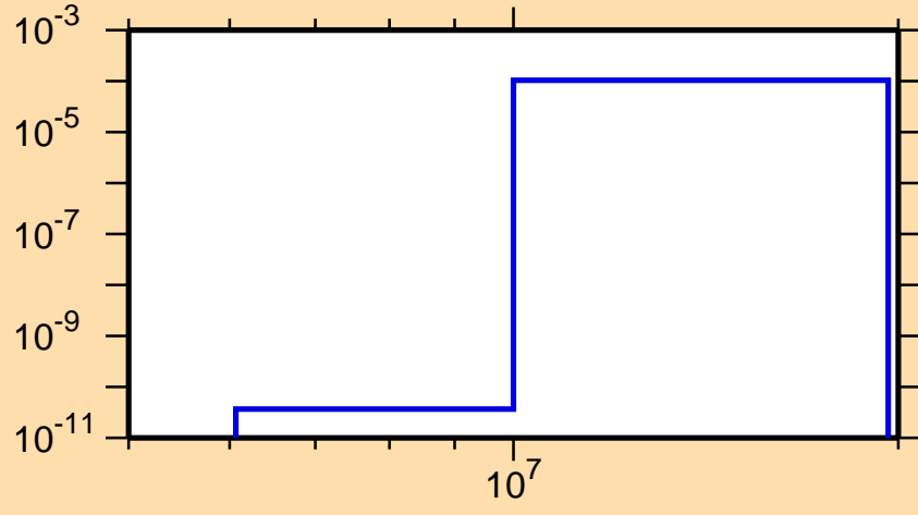
\sigma vs. E for ^{254}\text{Es}(n,np)
