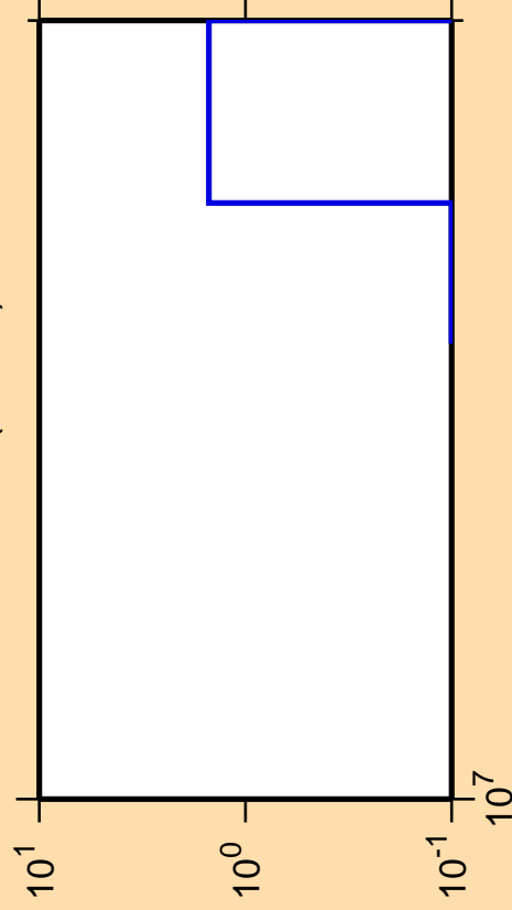
\Delta\sigma/\sigma vs. E for ^{255}\text{Es} (mt 42)
