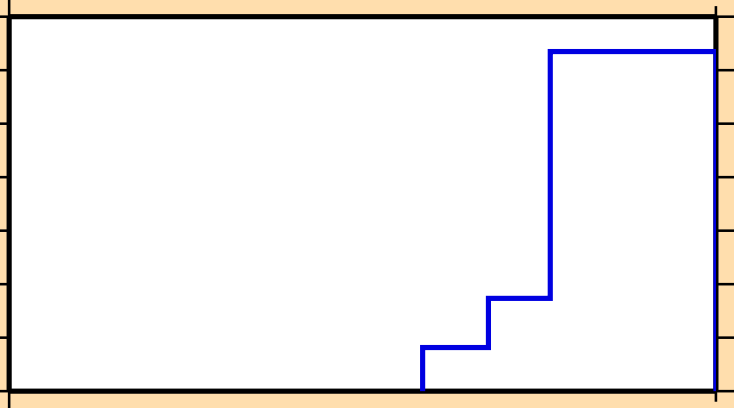
\sigma vs. E for ^{255}\text{Es} (mt 42)
