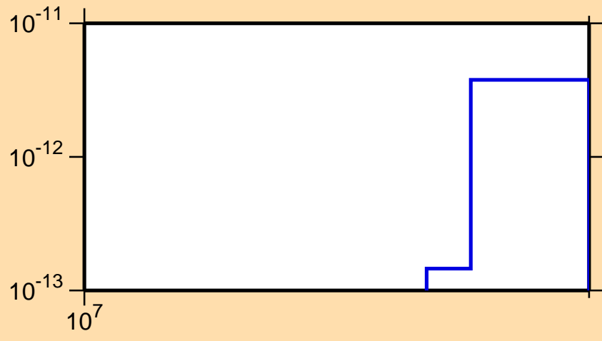
\sigma vs. E for ^{255}\text{Es}(n,\text{He3})
