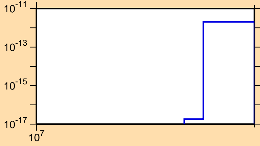
\sigma vs. E for ^{255}\text{Es} (mt 11)
