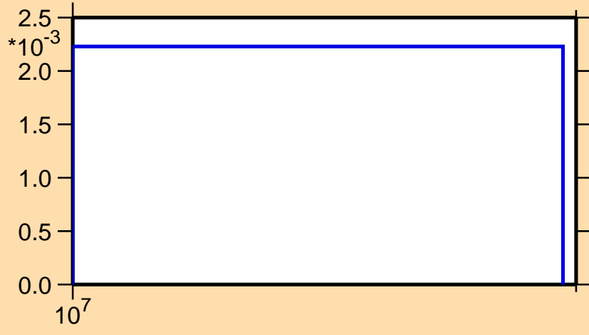
\sigma vs. E for ^{255}\text{Es}(n,3n)
