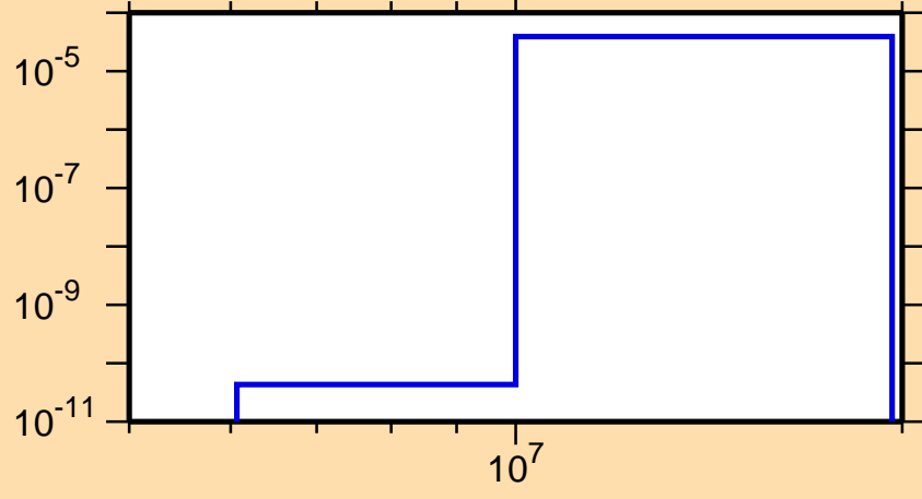
\sigma vs. E for ^{255}\text{Es}(n,np)
