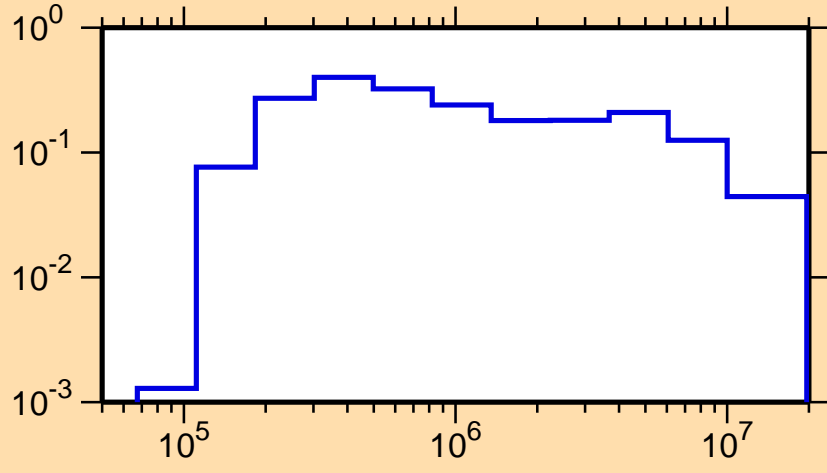
\sigma vs. E for ^{255}\text{Es}(n,n_1)
