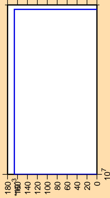
\Delta\sigma/\sigma vs. E for ^{255}\text{Es}(n,3n\alpha)
