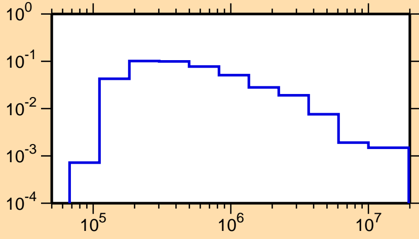
\sigma vs. E for ^{255}\text{Es}(n,n\text{cont.})
