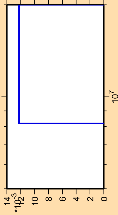
\Delta\sigma/\sigma vs. E for ^{255}\text{Es} (mt 42)
