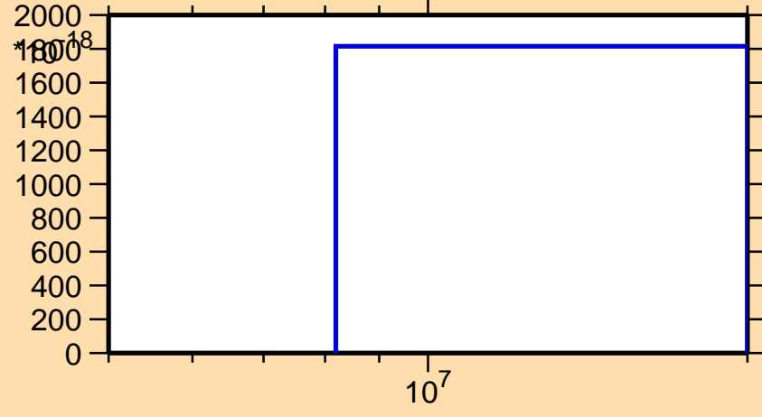
\sigma vs. E for ^{255}\text{Es} (mt 42)
