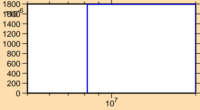
\sigma vs. E for ^{255}\text{Es}(n,3n)
