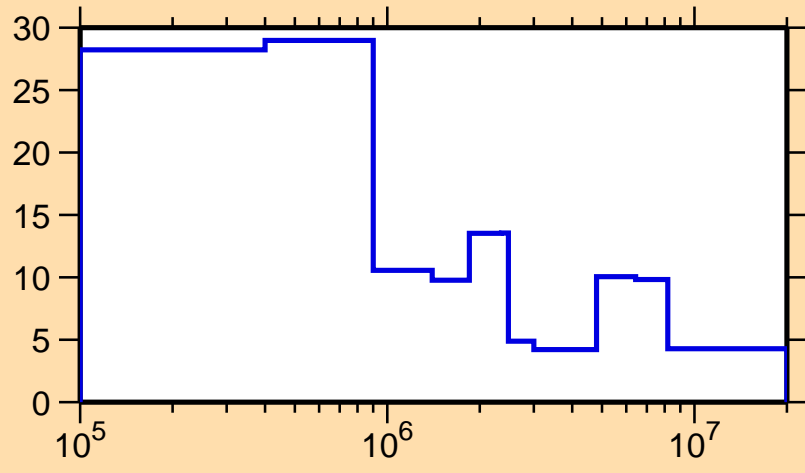
\Delta\sigma/\sigma vs. E for ^{255}\text{Es}(n,\text{tot.})
