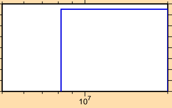
\sigma vs. E for ^{255}\text{Es}(n,\text{He3})
