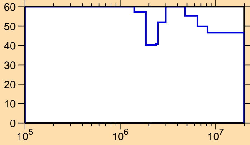
\Delta\sigma/\sigma vs. E for ^{255}\text{Es}(n,n_1)
