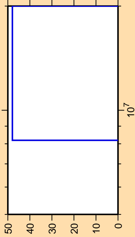
\Delta\sigma/\sigma vs. E for ^{255}\text{Es}(n,nt)
