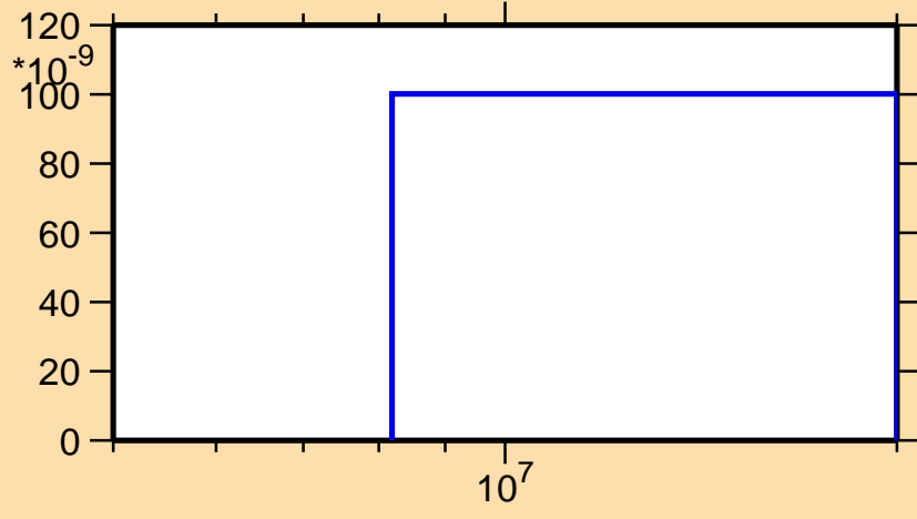
\sigma vs. E for ^{255}\text{Es}(n,nt)
