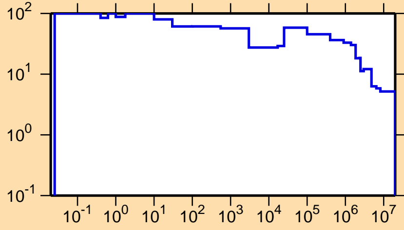
\Delta\sigma/\sigma vs. E for ^{255}\text{Es}(n,\text{nonel.})
