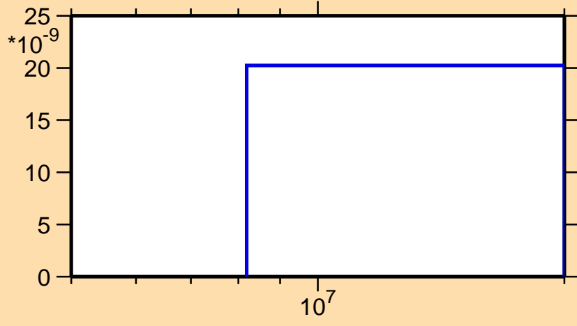
\sigma vs. E for ^{255}\text{Es}(n,2np)
