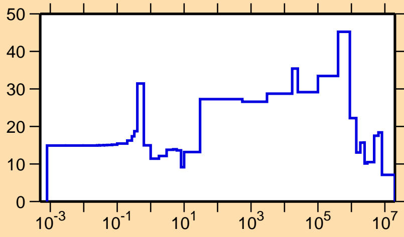
\Delta\sigma/\sigma vs. E for ^{255}\text{Es}(n,\text{el.})
