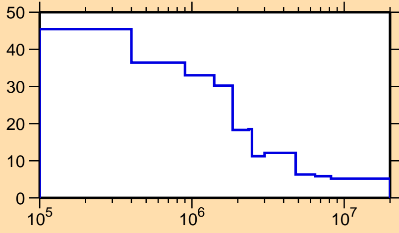
\Delta\sigma/\sigma vs. E for ^{255}\text{Es}(n,\text{nonel.})
