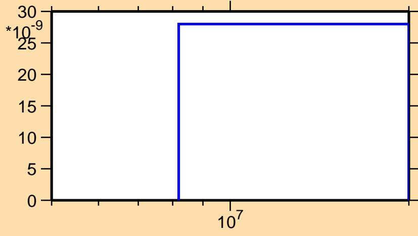
\sigma vs. E for ^{255}\text{Es}(n,nd)
