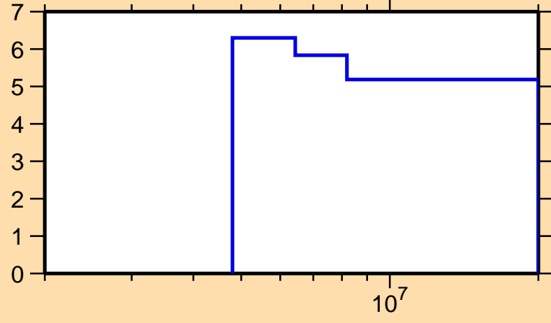
\Delta\sigma/\sigma vs. E for ^{255}\text{Es}(n,\text{nonel.})
