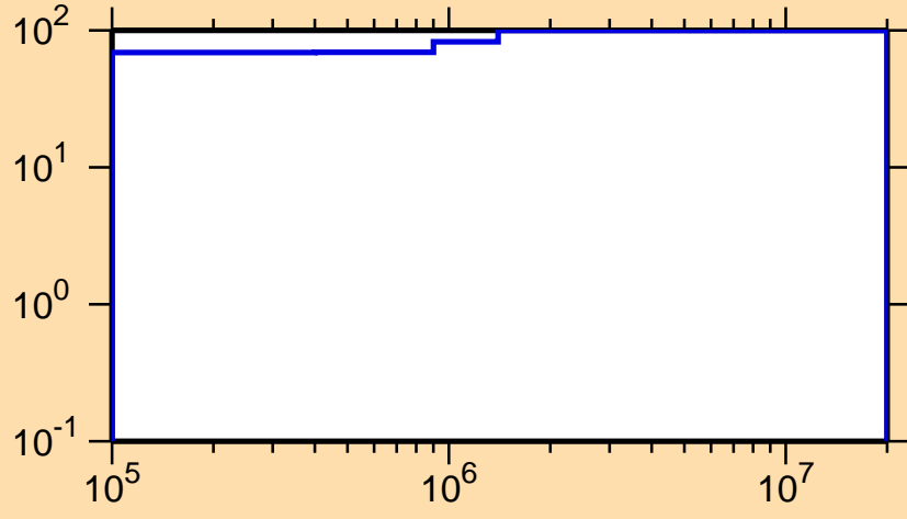
\Delta\sigma/\sigma vs. E for ^{255}\text{Es}(n,n\text{cont.})
