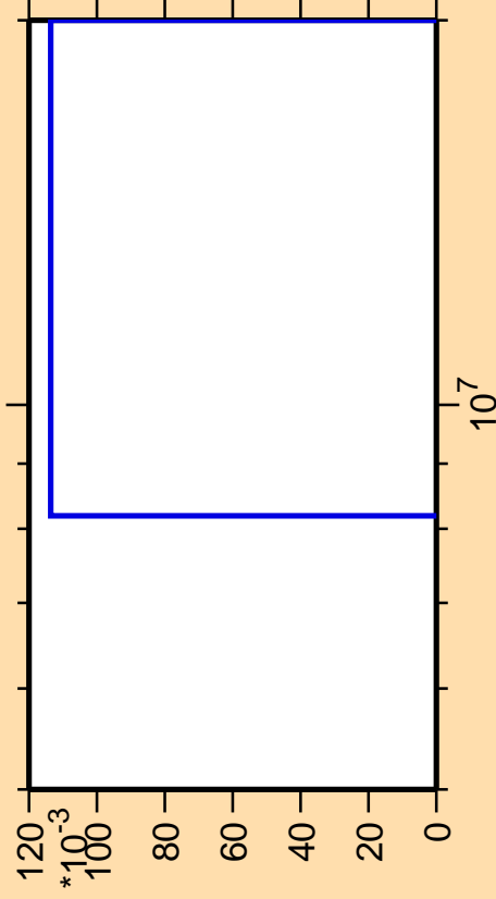
\Delta\sigma/\sigma vs. E for ^{255}\text{Es}(n,\text{He3})
