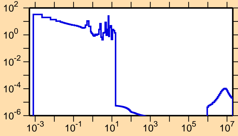
\sigma vs. E for ^{256}\text{Es}(n,\gamma)
