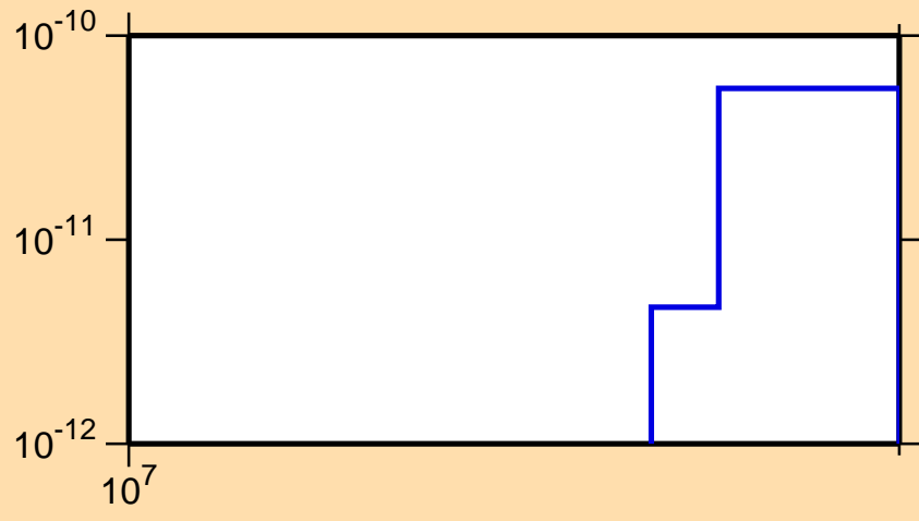
\sigma vs. E for ^{256}\text{Es}(n,3n\alpha)
