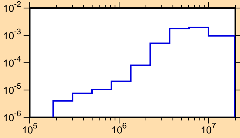
\sigma vs. E for ^{256}\text{Es}(n,n_1)
