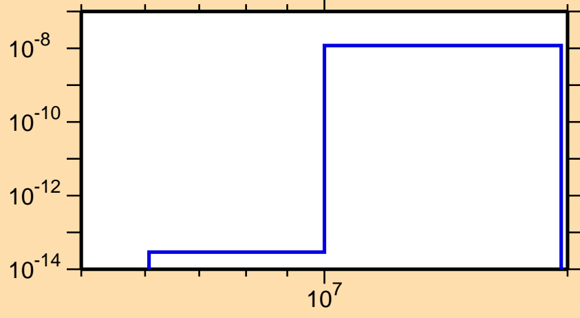
\sigma vs. E for ^{256}\text{Es}(n,2n\alpha)
