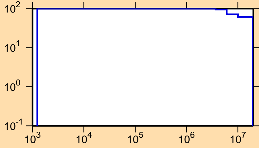
\Delta\sigma/\sigma vs. E for ^{256}\text{Es}(n,n\text{cont.})
