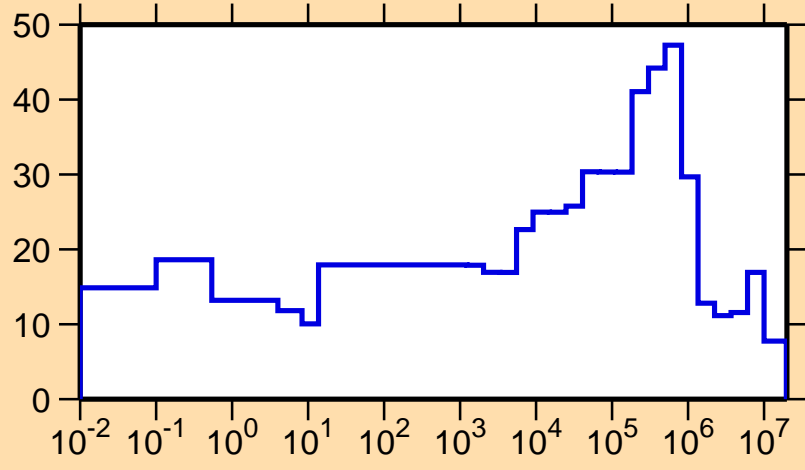
\Delta\sigma/\sigma vs. E for ^{256}\text{Es}(n,el.)
