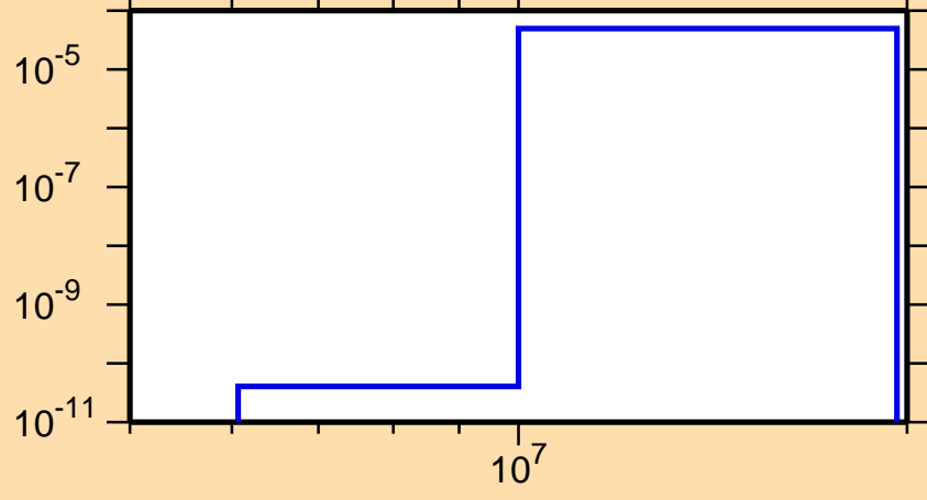
\sigma vs. E for ^{256}\text{Es}(n,np)
