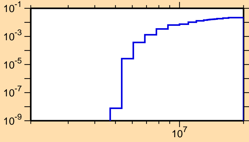
\sigma vs. E for ^{258}\text{Es}(n,2n)
