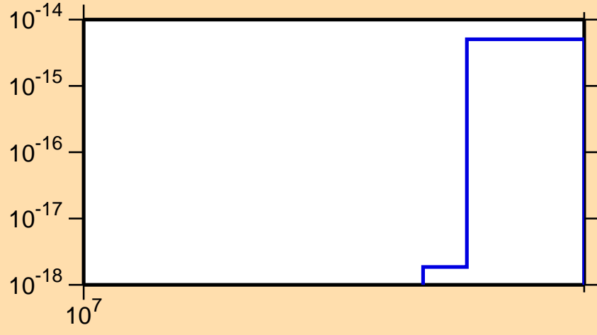
\sigma vs. E for ^{258}\text{Es}(n,3n\alpha)
