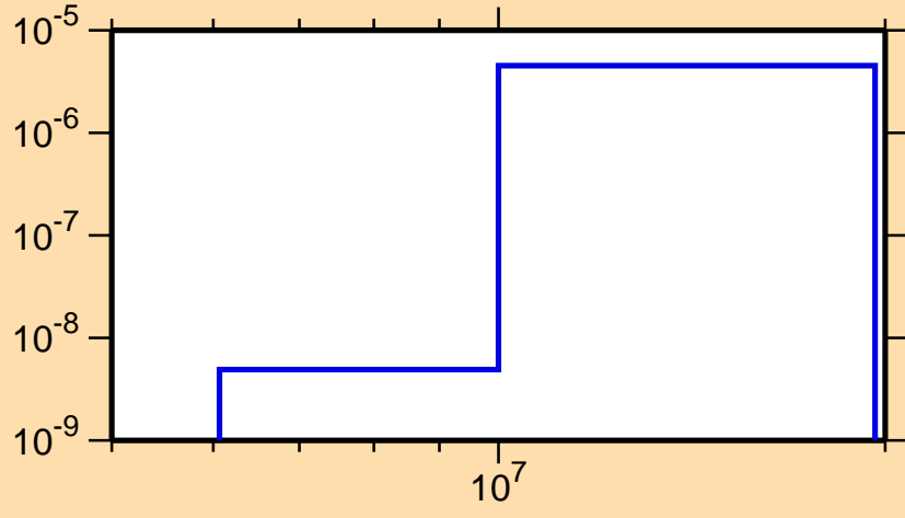
\sigma vs. E for ^{258}\text{Es}(n,n\alpha)
