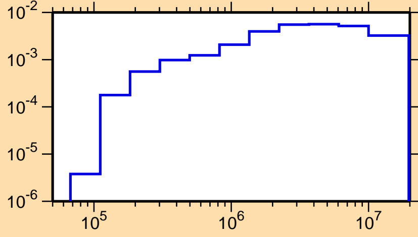
\sigma vs. E for ^{258}\text{Es}(n,\text{inel.})
