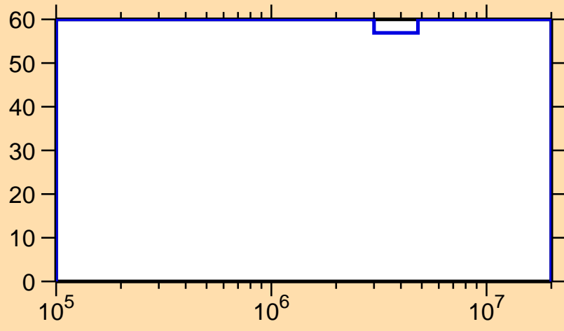
\Delta\sigma/\sigma vs. E for ^{258}\text{Es}(n,n_1)
