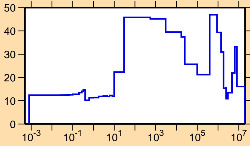
\Delta\sigma/\sigma vs. E for ^{258}\text{Es}(n,el.)
