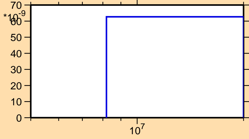
\sigma vs. E for ^{258}\text{Es}(n,nt)
