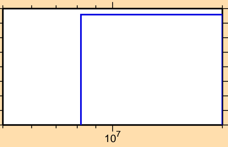
\sigma vs. E for ^{258}\text{Es}(n,\text{He3})
