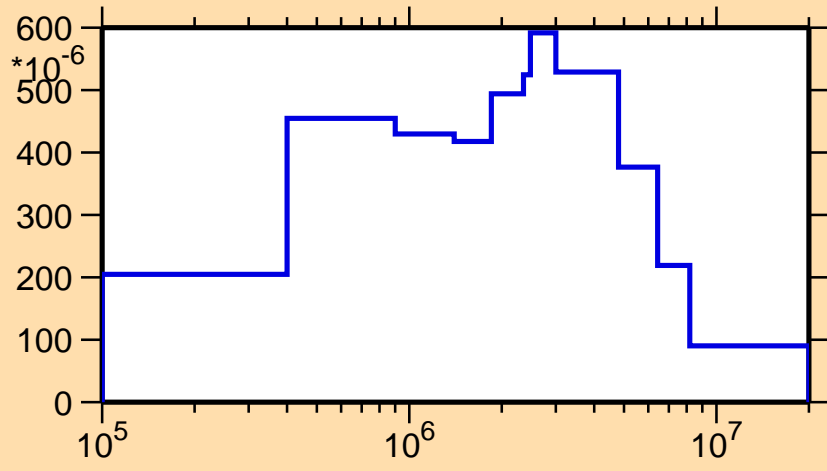
\sigma vs. E for ^{258}\text{Es}(n,n\text{cont.})
