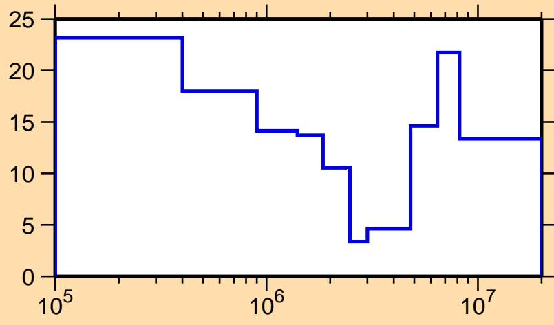
\Delta\sigma/\sigma vs. E for ^{258}\text{Es}(n,\text{tot.})
