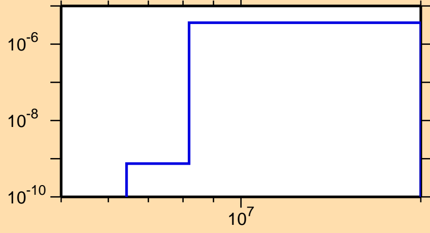
\sigma vs. E for ^{258}\text{Es}(n,n\alpha)
