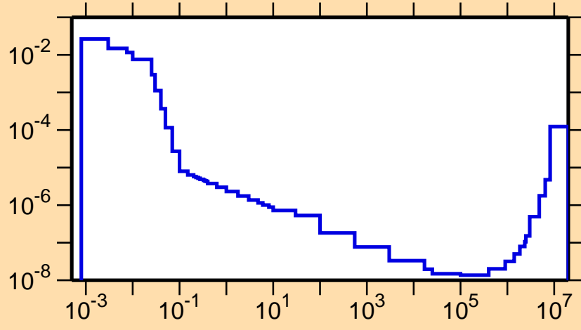
\sigma vs. E for ^{258}\text{Es}(n,\alpha)
