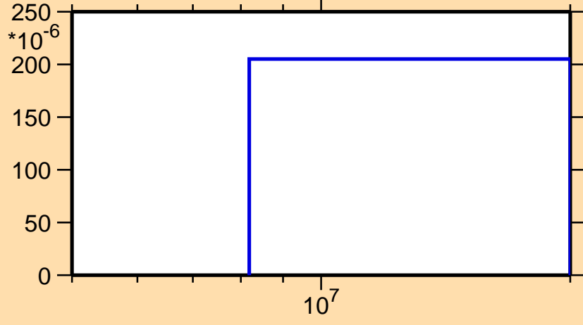
\sigma vs. E for ^{258}\text{Es}(n,np)
