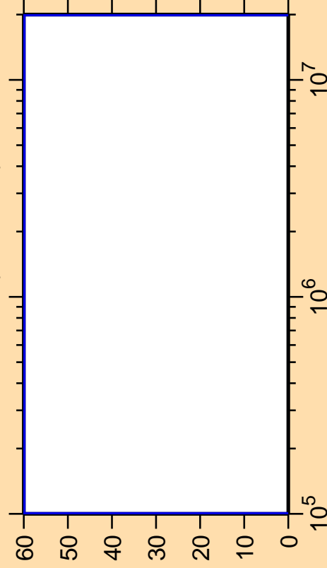
\Delta\sigma/\sigma vs. E for ^{258}\text{Es}(n,n\text{cont.})
