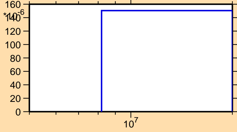
\sigma vs. E for ^{258}\text{Es}(n,d)
