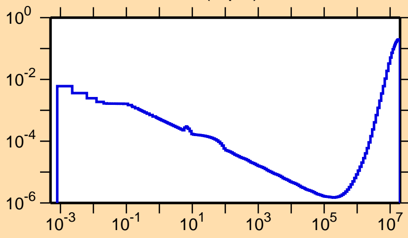
\sigma vs. E for ^{135}\text{Eu}(n,p\alpha)
