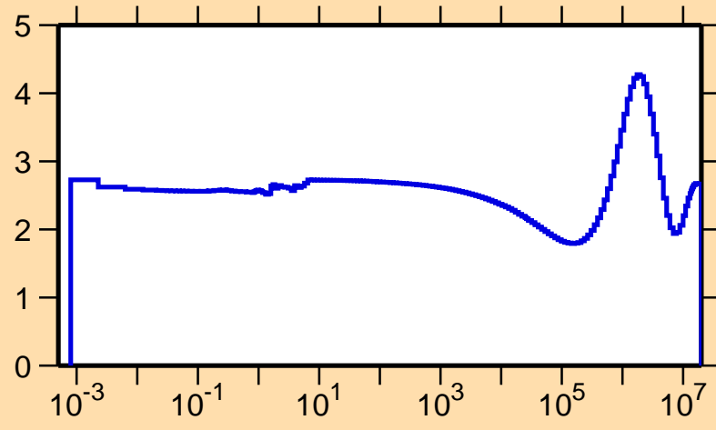
\sigma vs. E for ^{135}\text{Eu}(n,\text{el.})
