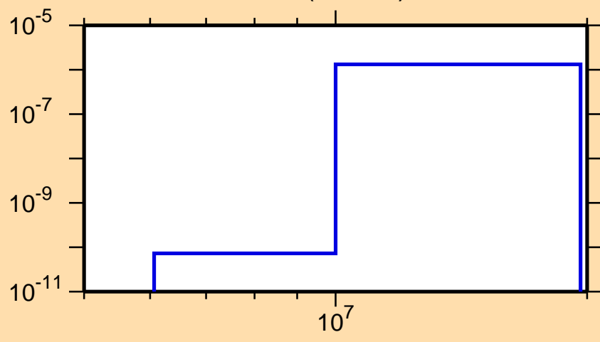
\sigma vs. E for ^{135}\text{Eu}(\text{mt117})
