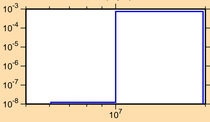
\sigma vs. E for ^{135}\text{Eu}(n,\text{pd})
