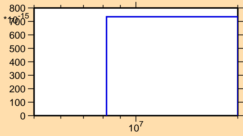
\sigma vs. E for ^{135}\text{Eu}(n,2n\alpha)
