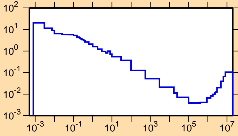
\sigma vs. E for ^{135}\text{Eu}(n,\alpha)
