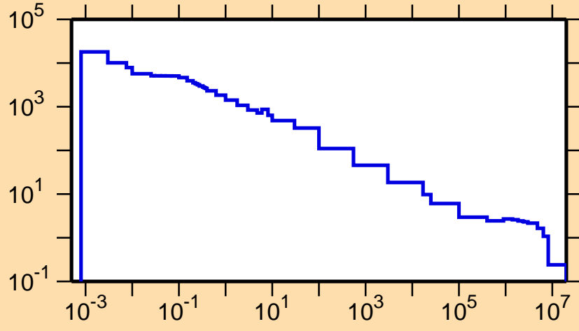
\sigma vs. E for ^{135}\text{Eu}(n,p)
