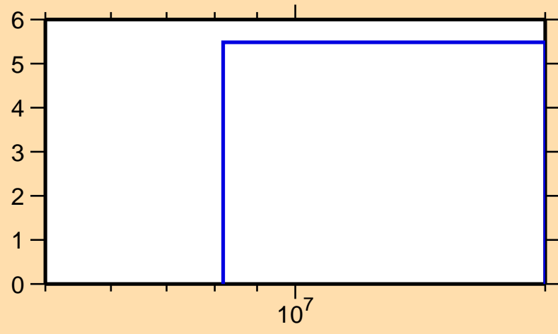
\Delta\sigma/\sigma vs. E for ^{135}\text{Eu}(n,\text{el.})
