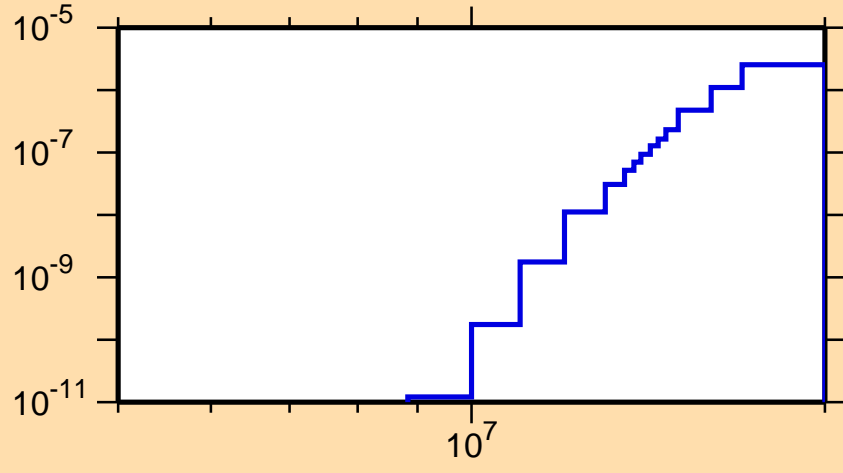
\sigma vs. E for ^{136}\text{Eu}(\text{mt117})
