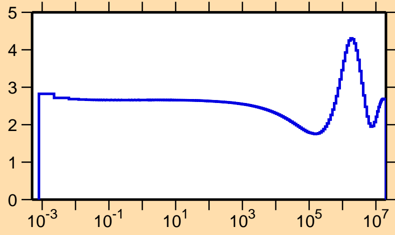
\sigma vs. E for ^{136}\text{Eu}(n,\text{el.})
