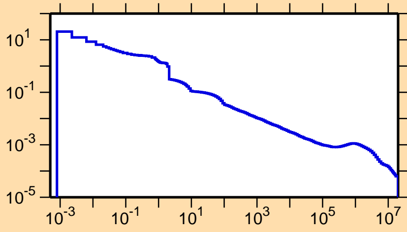
\sigma vs. E for ^{136}\text{Eu}(n,\gamma)
