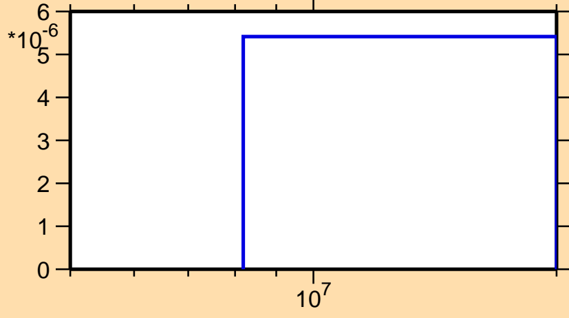
\sigma vs. E for ^{136}\text{Eu}(n,nd)
