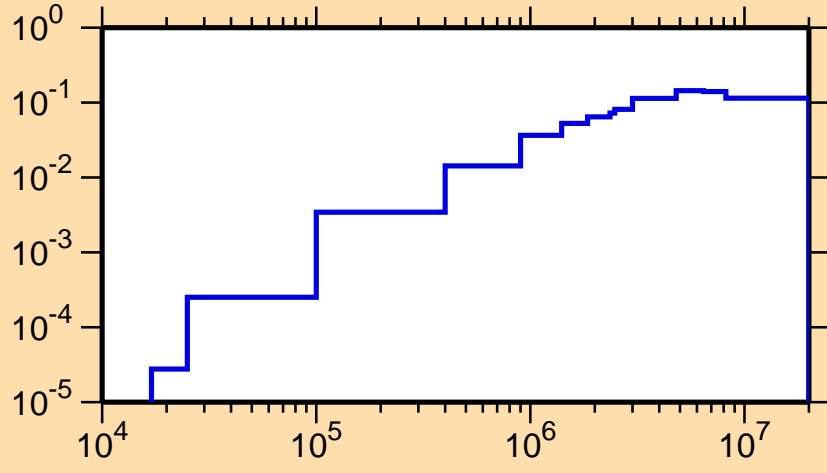
\sigma vs. E for ^{136}\text{Eu}(n,n\text{cont.})
