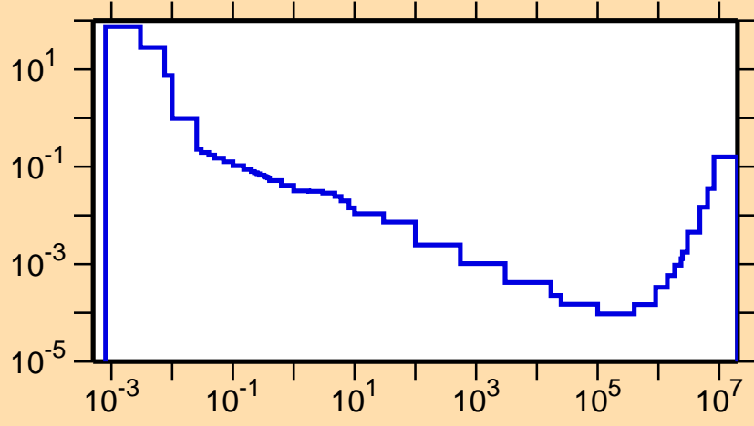
\sigma vs. E for ^{136}\text{Eu}(n,p\alpha)
