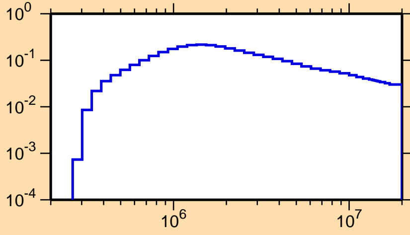
\sigma vs. E for ^{137}\text{Eu}(n,n_1)
