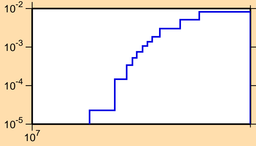
\sigma vs. E for ^{137}\text{Eu}(n,2n)
