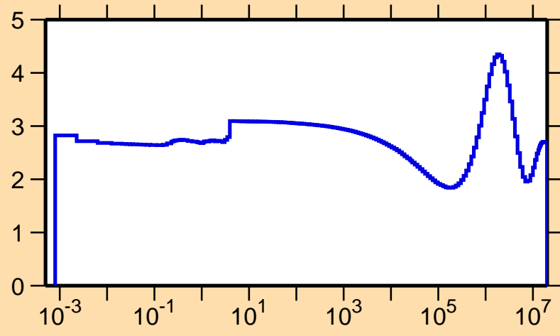
\sigma vs. E for ^{137}\text{Eu}(n,\text{el.})
