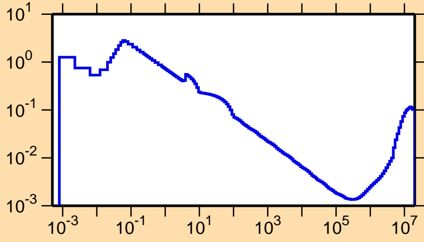
\sigma vs. E for ^{137}\text{Eu}(n,\alpha)
