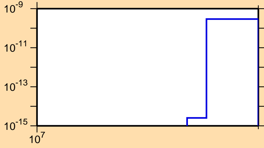
\sigma vs. E for ^{137}\text{Eu}(n,nt)
