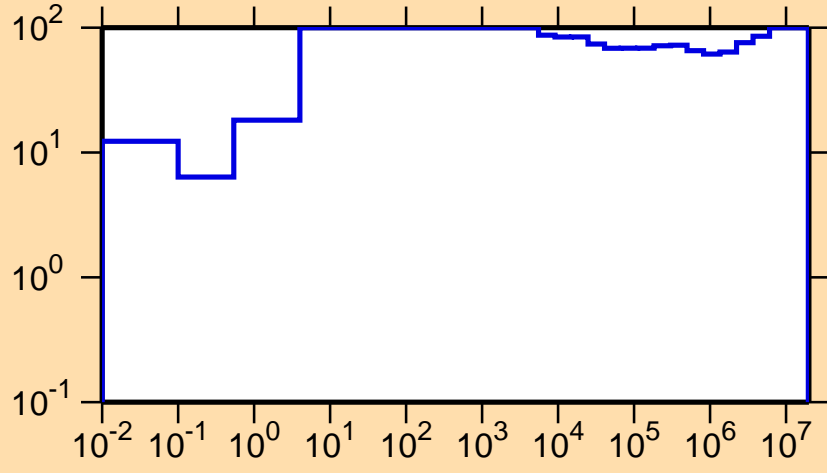
\Delta\sigma/\sigma vs. E for ^{137}\text{Eu}(n,\gamma)
