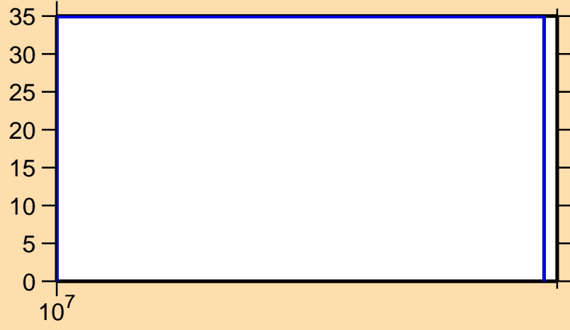
\Delta\sigma/\sigma vs. E for ^{137}\text{Eu}(n,\text{inel.})
