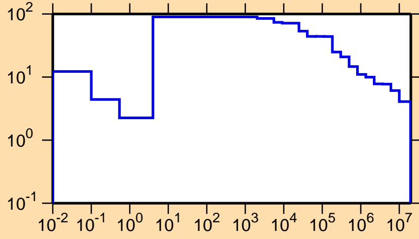
\Delta\sigma/\sigma vs. E for ^{137}\text{Eu}(n,\text{tot.})
