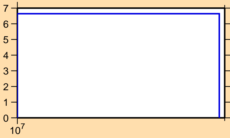
\Delta\sigma/\sigma vs. E for ^{137}\text{Eu}(n,\text{nonel.})
