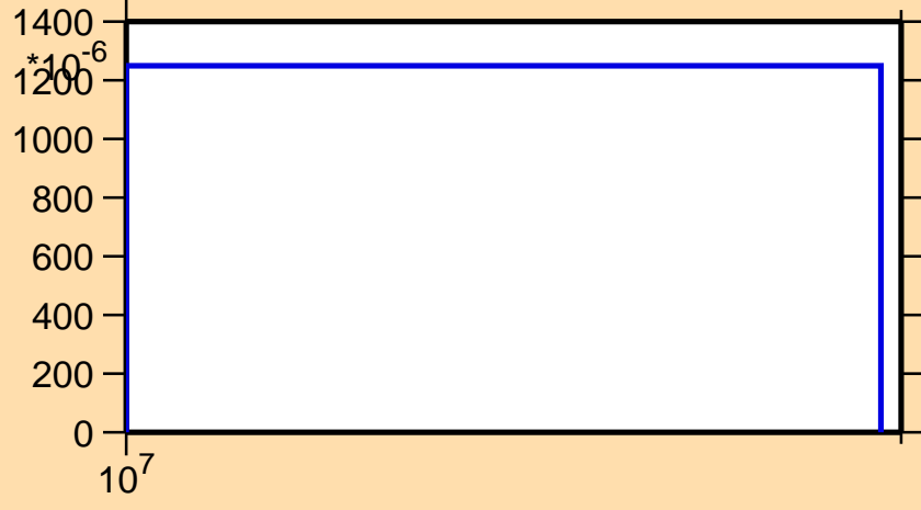
\sigma vs. E for ^{137}\text{Eu}(n,2n)
