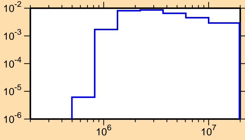
\sigma vs. E for ^{137}\text{Eu}(n,n_2)
