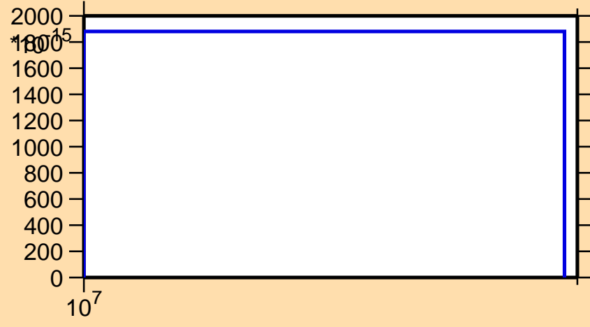
\sigma vs. E for ^{137}\text{Eu}(n,nt)
