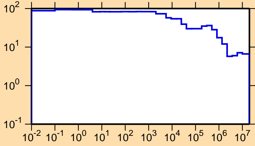
\Delta\sigma/\sigma vs. E for ^{137}\text{Eu}(n,\text{nonel.})
