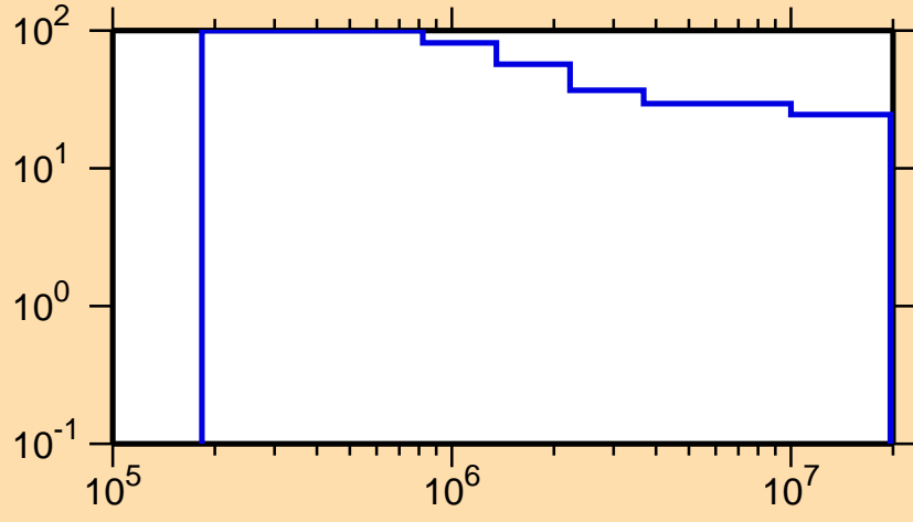
\Delta\sigma/\sigma vs. E for ^{137}\text{Eu}(n,n_1)
