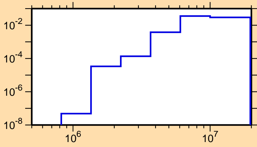
\sigma vs. E for ^{137}\text{Eu}(n,n\text{cont.})
