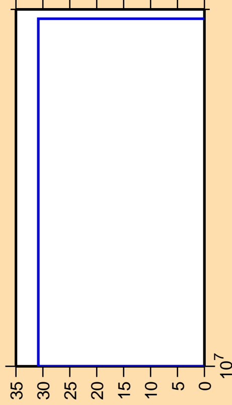
\Delta\sigma/\sigma vs. E for ^{137}\text{Eu} (mt 34)
