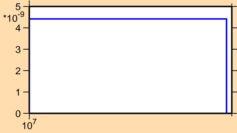
\sigma vs. E for ^{137}\text{Eu}(n,pt)
