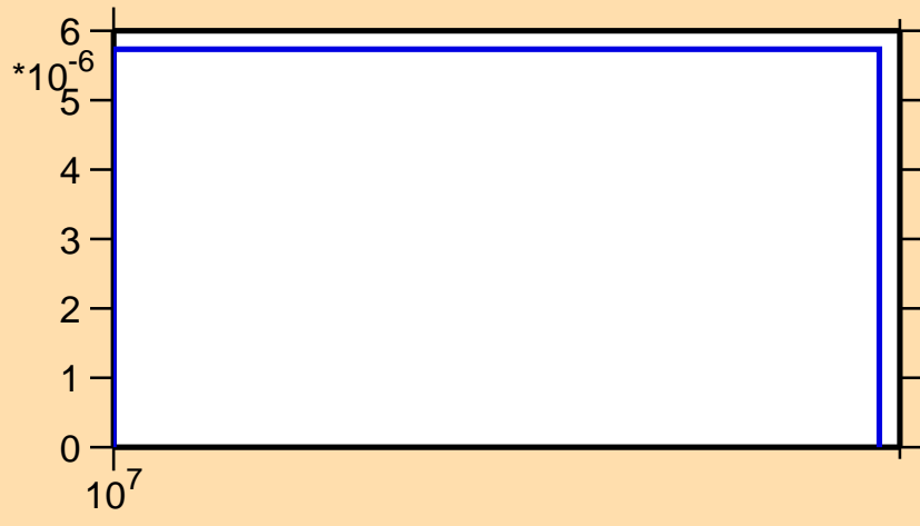
\sigma vs. E for ^{137}\text{Eu}(n,2np)
