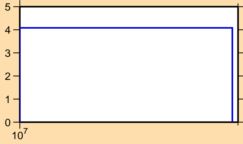
\Delta\sigma/\sigma vs. E for ^{137}\text{Eu}(n,\text{tot.})
