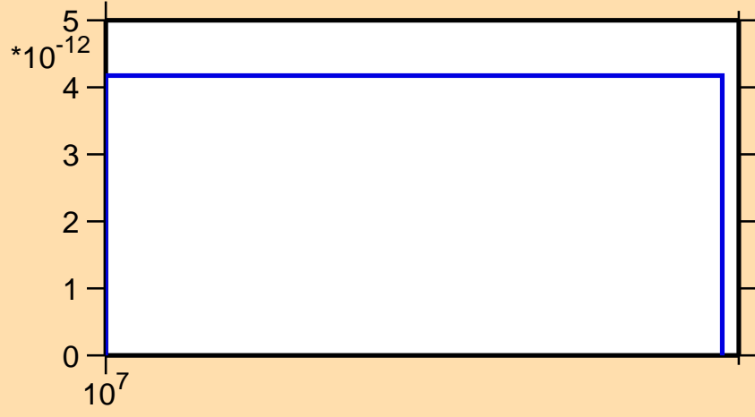
\sigma vs. E for ^{137}\text{Eu} (mt 34)
