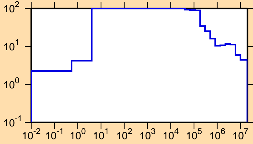
\Delta\sigma/\sigma vs. E for ^{137}\text{Eu}(n,\text{el.})
