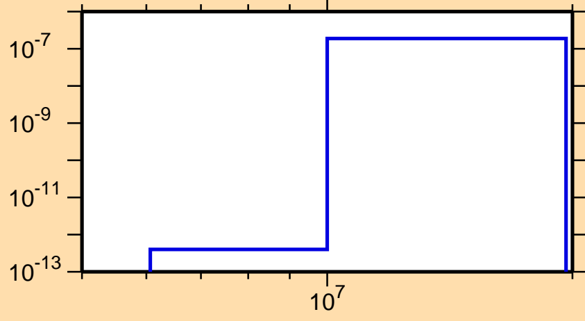
\sigma vs. E for ^{137}\text{Eu}(\text{mt117})
