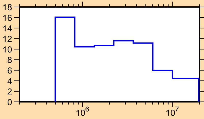
\Delta\sigma/\sigma vs. E for ^{137}\text{Eu}(n, \text{el.})
