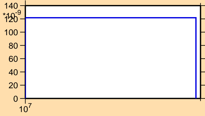
\sigma vs. E for ^{137}\text{Eu}(n,nd)
