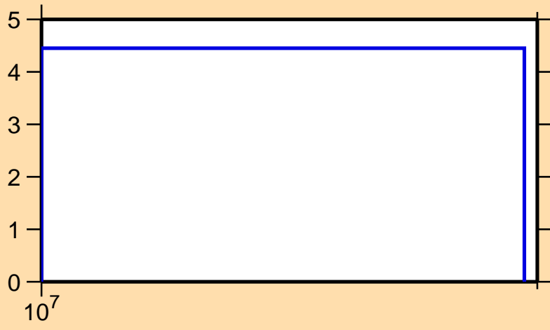
\Delta\sigma/\sigma vs. E for ^{137}\text{Eu}(n,\text{el.})
