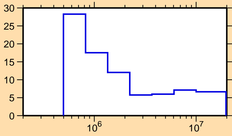
\Delta\sigma/\sigma vs. E for ^{137}\text{Eu}(n,\text{nonel.})
