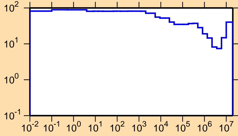
\Delta\sigma/\sigma vs. E for ^{137}\text{Eu}(n,p)
