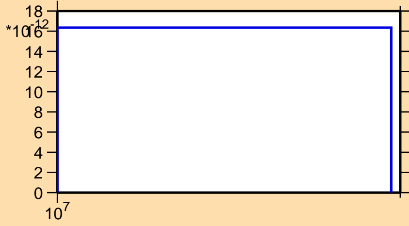
\sigma vs. E for ^{137}\text{Eu}(n,2n\alpha)
