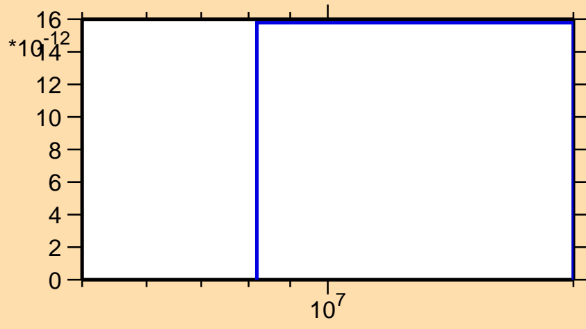
\sigma vs. E for ^{137}\text{Eu}(n,2n\alpha)
