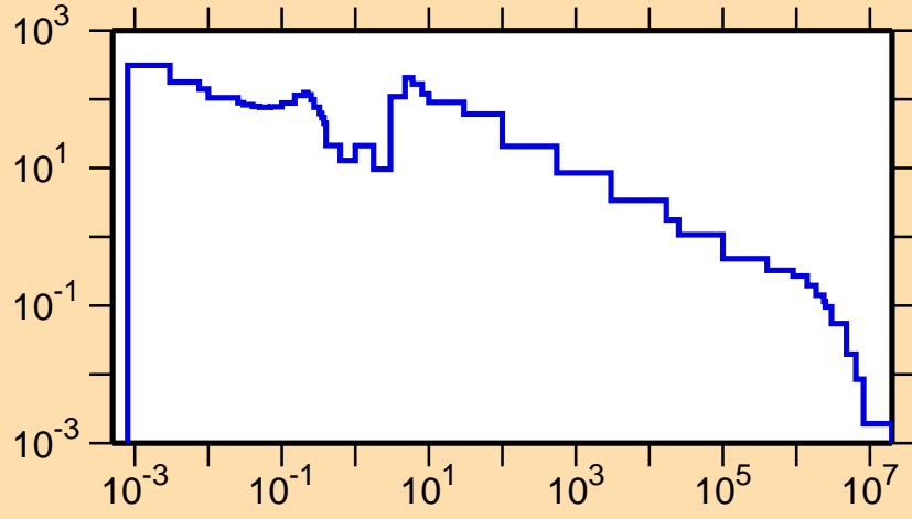
\sigma vs. E for ^{137}\text{Eu}(n,\gamma)
