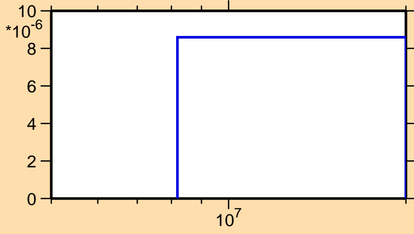
\sigma vs. E for ^{137}\text{Eu}(n,\text{pd})
