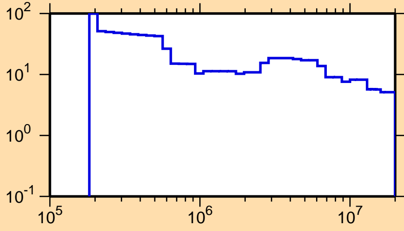
\Delta\sigma/\sigma vs. E for ^{138}\text{Eu}(n, el.)
