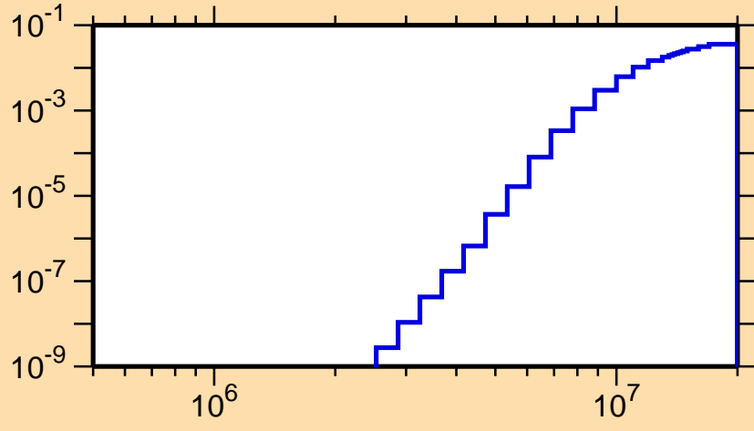
\sigma vs. E for ^{138}\text{Eu}(n,d)
