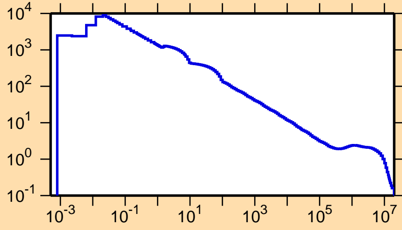
\sigma vs. E for ^{138}\text{Eu}(n,p)
