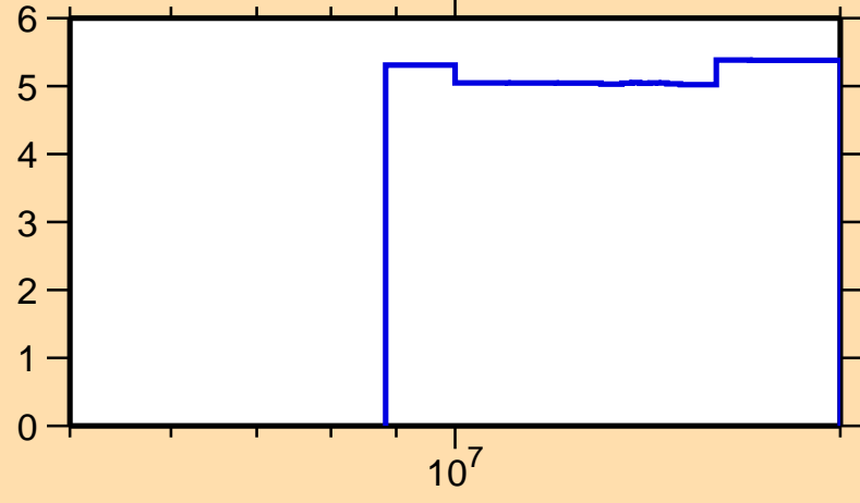
\Delta\sigma/\sigma vs. E for ^{138}\text{Eu}(n,\text{tot.})
