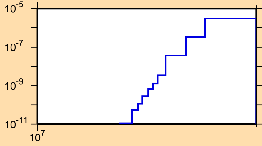
\sigma vs. E for ^{138}\text{Eu}(n,pt)
