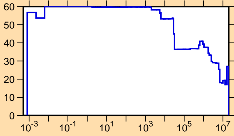
\Delta\sigma/\sigma vs. E for ^{138}\text{Eu}(n,p)
