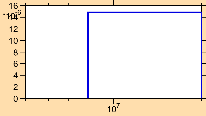
\sigma vs. E for ^{138}\text{Eu} (mt 45)
