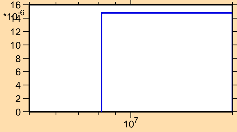
\sigma vs. E for ^{138}\text{Eu}(n,\text{pd})
