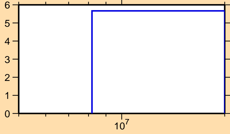
\Delta\sigma/\sigma vs. E for ^{138}\text{Eu}(n,\text{el.})
