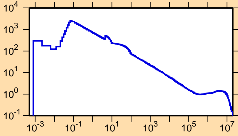
\sigma vs. E for ^{139}\text{Eu}(n,p)
