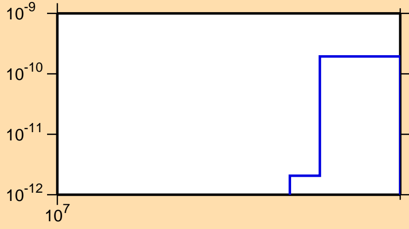
\sigma vs. E for ^{139}\text{Eu} (mt 34)
