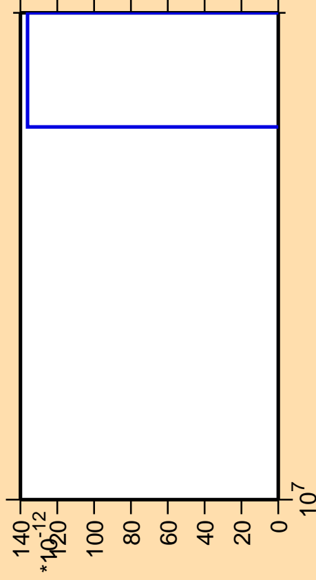
\Delta\sigma/\sigma vs. E for ^{139}\text{Eu} (mt 11)
