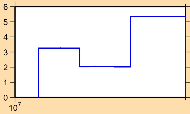
\Delta\sigma/\sigma vs. E for ^{139}\text{Eu}(n,\text{tot.})
