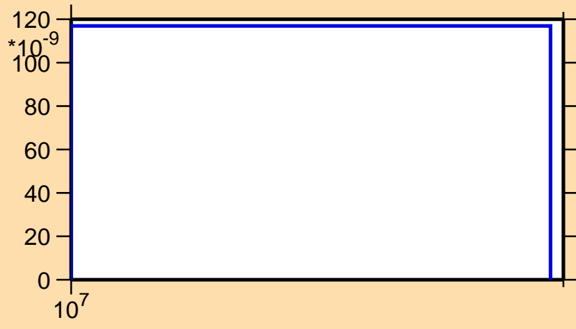
\sigma vs. E for ^{139}\text{Eu}(n,\text{nd})
