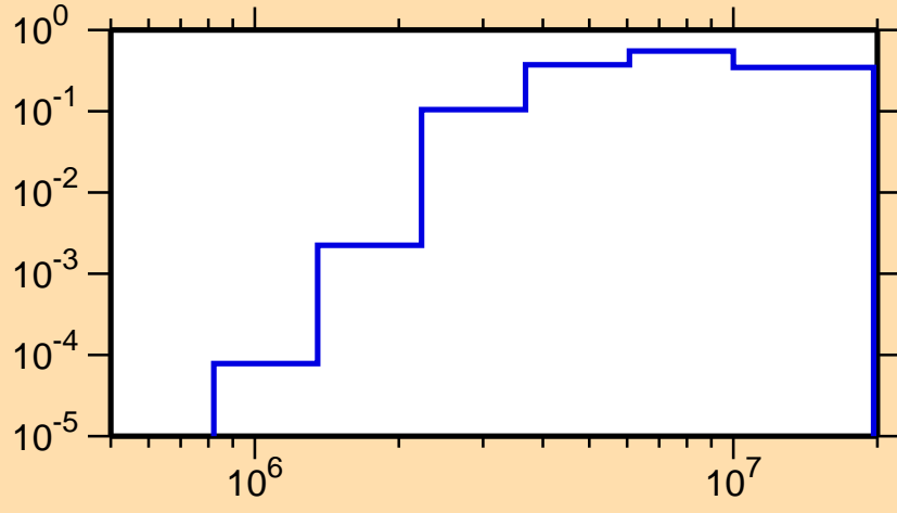
\sigma vs. E for ^{139}\text{Eu}(n,n\text{cont.})
