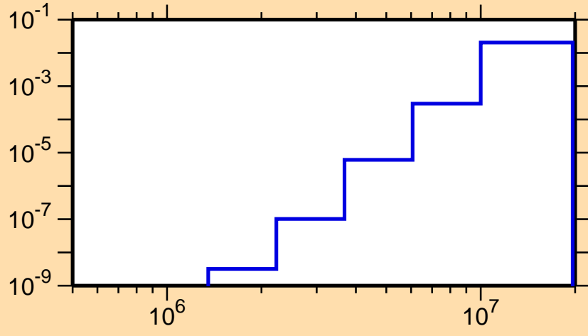
\sigma vs. E for ^{139}\text{Eu}(n,p\alpha)
