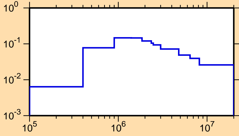
\sigma vs. E for ^{139}\text{Eu}(n,n_4)
