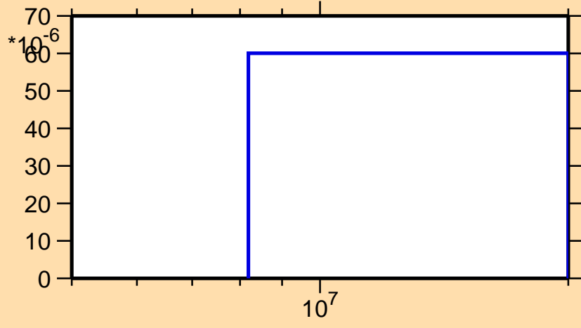
\sigma vs. E for ^{139}\text{Eu} (mt 45)
