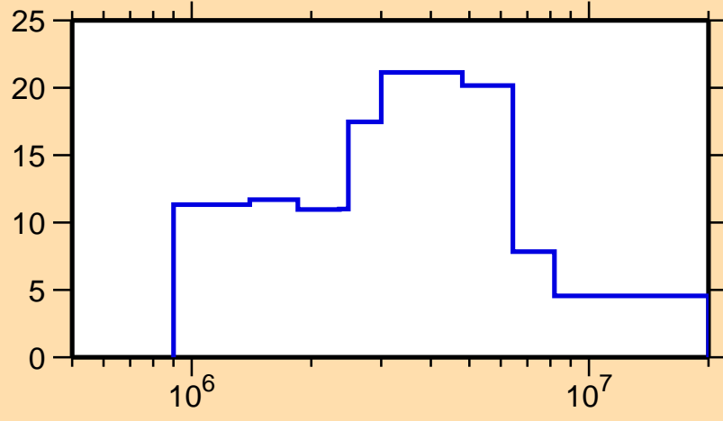
\Delta\sigma/\sigma vs. E for ^{139}\text{Eu}(n, \text{el.})
