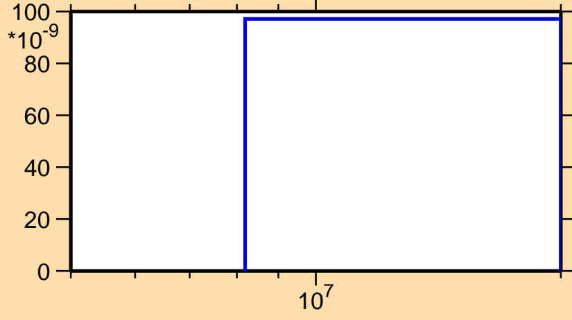
\sigma vs. E for ^{139}\text{Eu}(n,nd)
