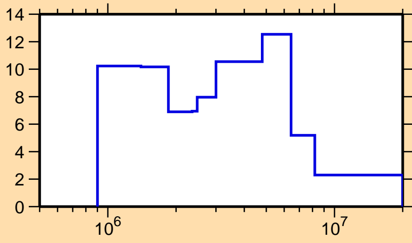
\Delta\sigma/\sigma vs. E for ^{139}\text{Eu}(n,\text{tot.})
