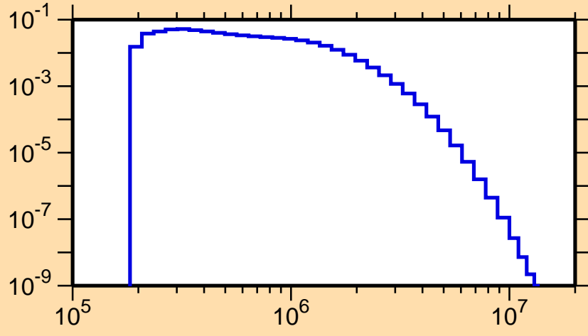
\sigma vs. E for ^{140}\text{Eu}(n,n_3)
