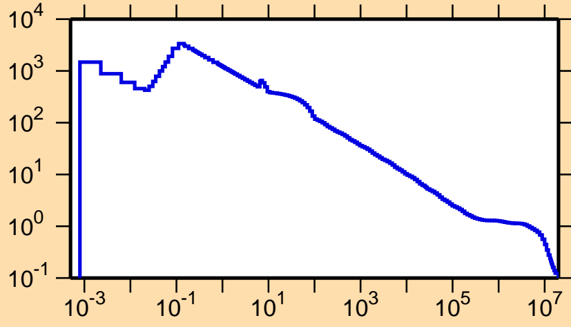
\sigma vs. E for ^{140}\text{Eu}(n,p)
