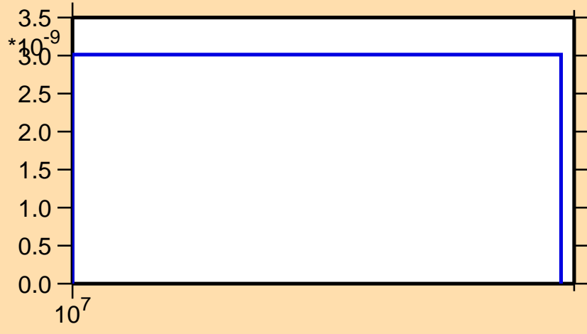
\sigma vs. E for ^{140}\text{Eu}(n,2n\alpha)
