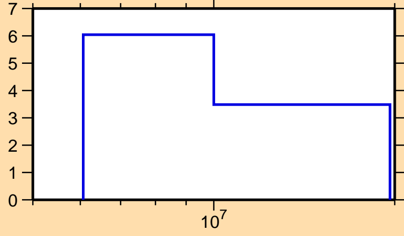
\Delta\sigma/\sigma vs. E for ^{140}\text{Eu}(n,\text{tot.})
