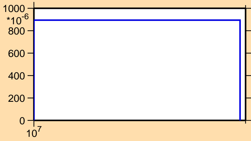
\sigma vs. E for ^{140}\text{Eu}(n,2np)
