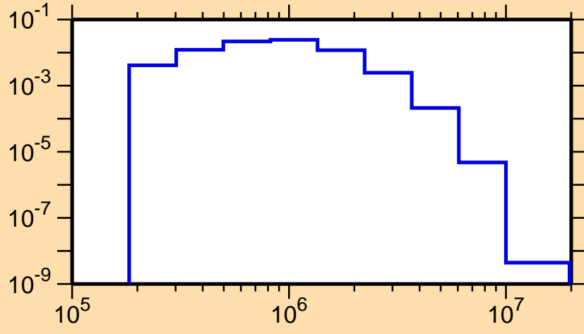
\sigma vs. E for ^{140}\text{Eu}(n,n_2)
