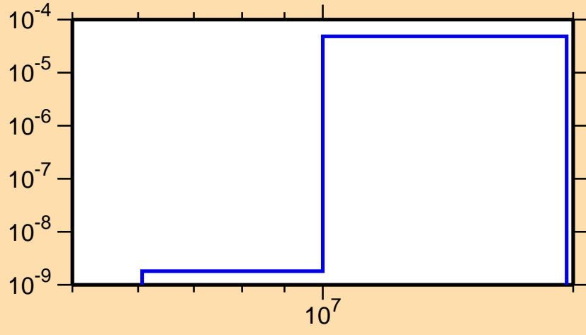
\sigma vs. E for ^{140}\text{Eu}(n,\text{He3})
