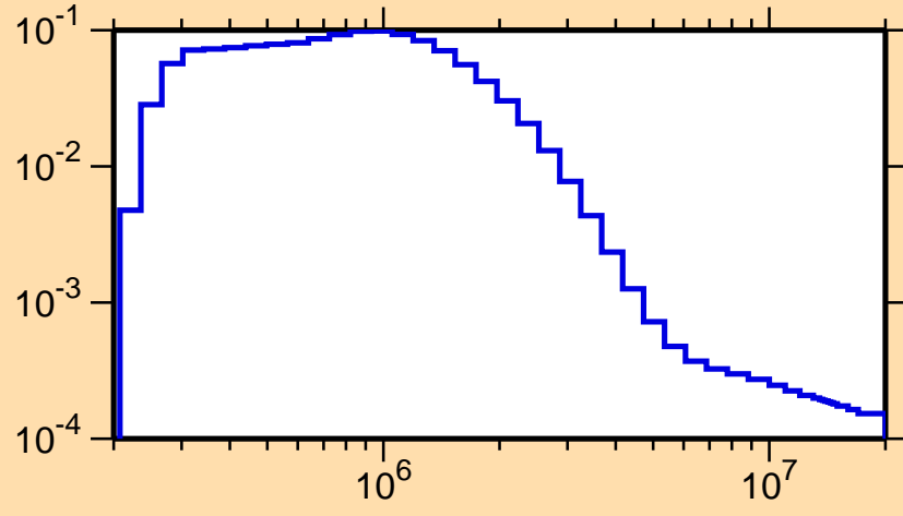
\sigma vs. E for ^{141}\text{Eu}(n,n_2)
