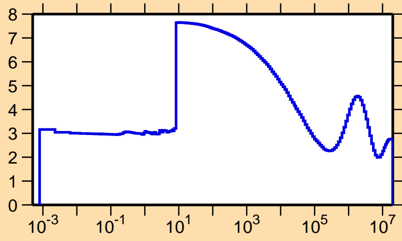
\sigma vs. E for ^{141}\text{Eu}(n,\text{el.})
